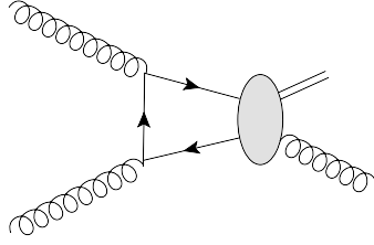
FIG. 4: One of the 2 Feynman diagrams for g g \rightarrow J/\psi g at order g_s^2 with vertex \Gamma_{\mu\nu} in the model for the s -channel cut contribution introduced in Ref. [4].
