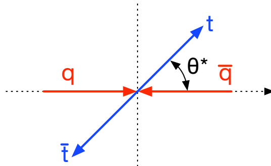
Figure 2: Production angle \theta^* in a q\bar{q} \rightarrow t\bar{t} event defined in the t\bar{t} center-of-mass frame.
