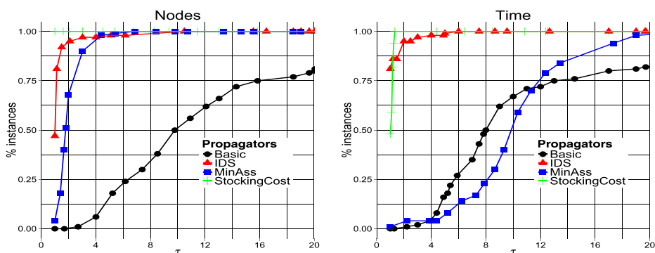
Fig. 12 Performance profiles: StockingCost , IDS , MinAss and Basic
