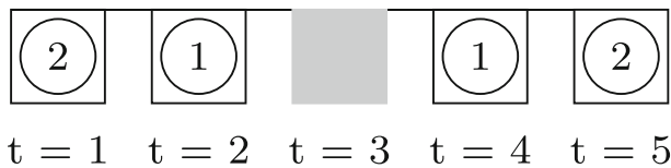
Fig. 10 An optimal solution of the PSP instance of Example 6
