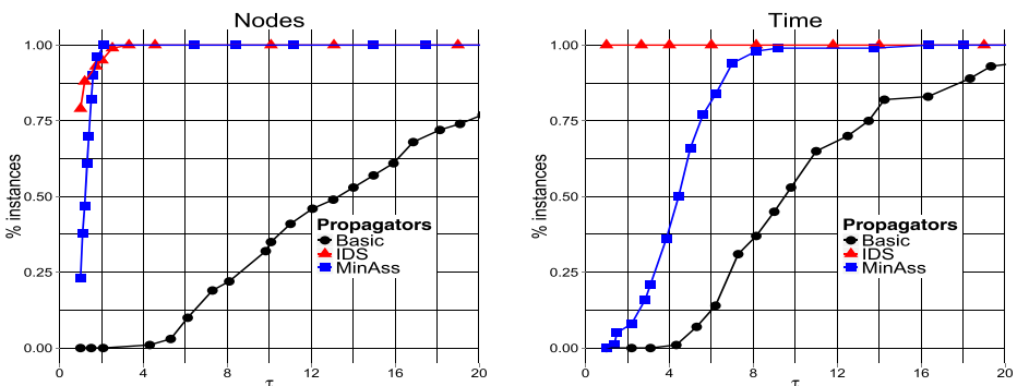
Fig. 11 Performance profiles: IDS , MinAss and Basic
