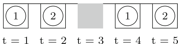
Fig. 9 A feasible solution of the PSP instance of Example 6
