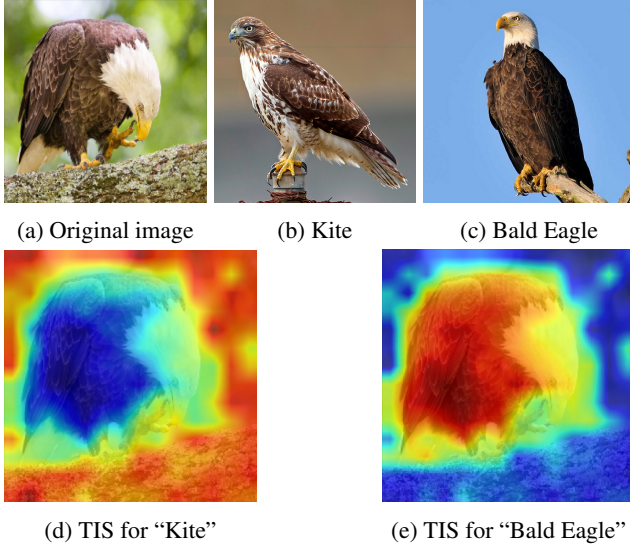
Figure 3: Class mismatch between the target and predicted class. 3a is the original image. The dataset target class is “Kite” while the model predicts “Bald Eagle”. For illustration purposes, 3b and 3c display other images of a Kite and a Bald Eagle, respectively. 3d is the saliency map produced by TIS for class “Kite” (dataset target) and 3e is the TIS saliency map for the model predicted class “Bald Eagle”.
