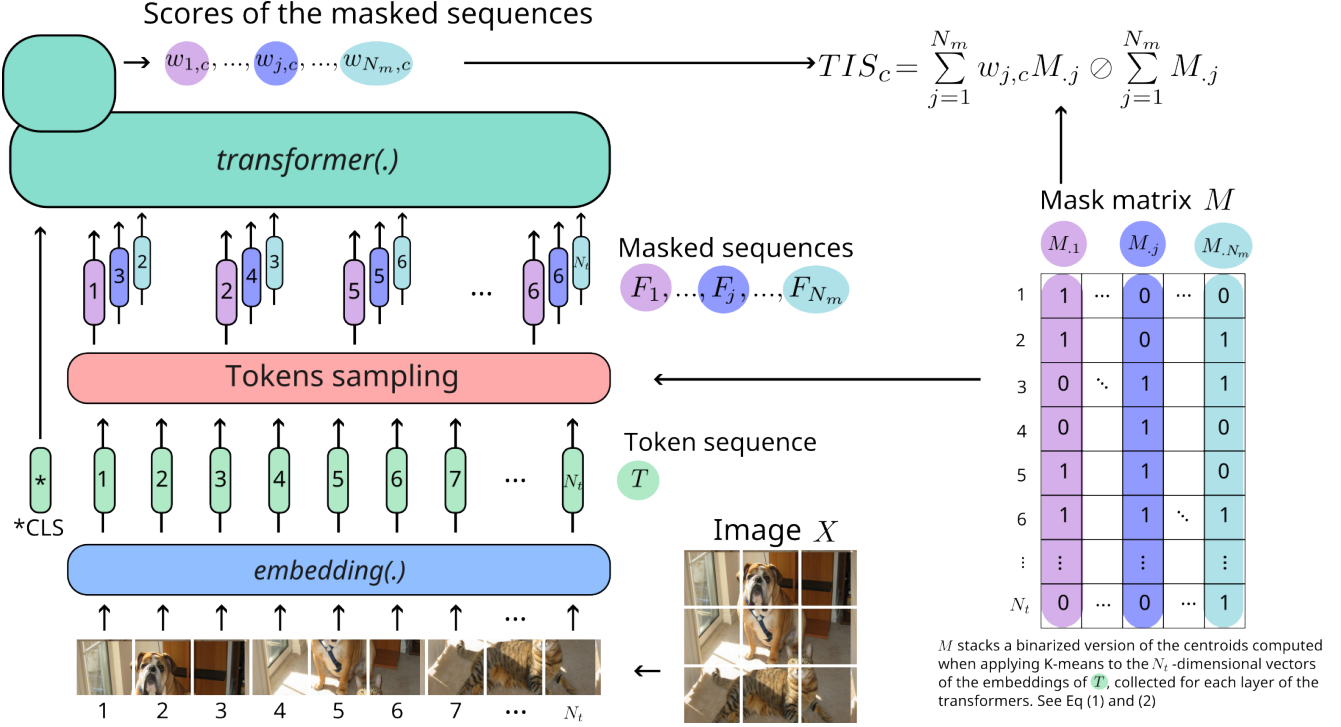
Figure 1: Illustration of the Transformer Input Sampling (TIS) process. The columns M_{.j} of the matrix M are the masks used to produce each sampled sequences F_j . The scores w_{j,c} are the scores for each sequences F_j for a target class c .
