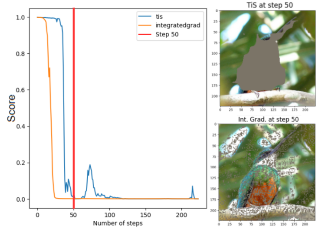
Figure 4: Comparison of TIS and Integrated Gradients results after 50 steps of the deletion metric. The target class is a jacamar (bird). Integrated Gradient perturbs the image diffusely, resulting in a better metric while still keeping the bird visible. On the other hand, TIS masks the bird itself, even though it may take more steps to reduce the target score.
