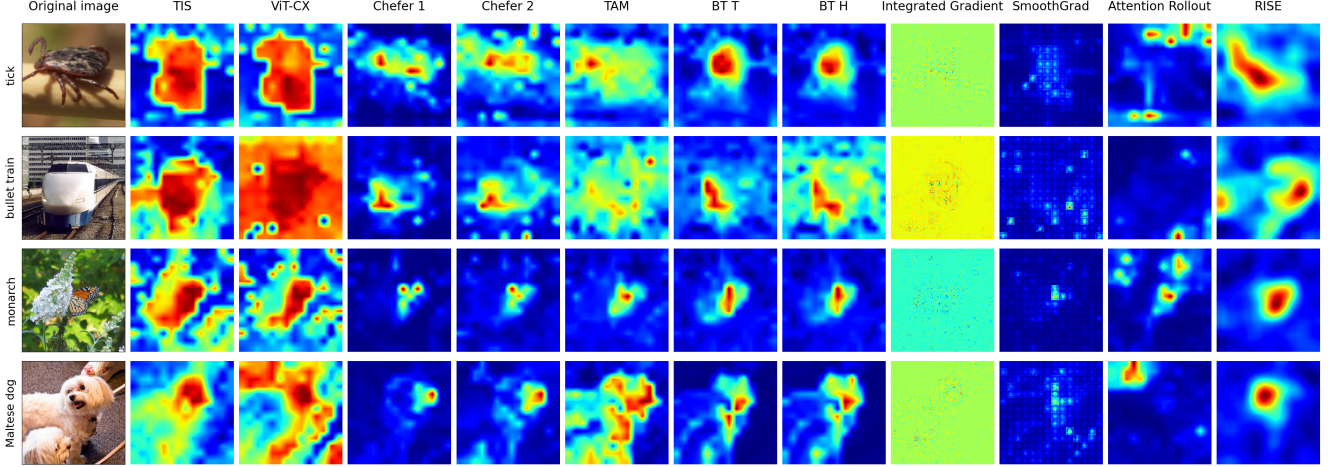
Figure 2: Comparison of the explainability methods for the ViT-Base model [7] on four random images from the ImageNet Validation set [19].
