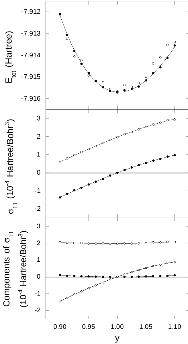
FIG. 10. Total energy (top) and \sigma_{11} (middle) of Si calculated at constant cut-off energy ( E_{cut}=6 Hartree with 2 special k -points in the IBZ) for 17 values of the ratio y = b/c in the case of an anisotropic deformation which consists in compressing (or expanding) the unit cell along the [001] direction in order that the length of the three cubic directions are changed to a = b and c keeping the volume V unchanged. The open circles ( \circ ) represent the uncorrected values, whereas the solid circles ( \bullet ) are the values corrected by the S.H. technique. The solid curves are obtained by least-squares third-order fit. The graph points out the effect of the correction, namely, the cancellation of the jumps between the micro-curves for energy, and a shift of the curve for stress. A decomposition of \sigma_{11} into its different components is also presented (bottom). The open circles ( \circ ) represent the uncorrected values of isotropic part of \sigma_{11} , whereas the solid circles ( \bullet ) are the values corrected by the S.H. technique. The open diamonds ( \diamond ) illustrate the values of the anisotropic part of \sigma_{11} , that are not affected by the correction.
