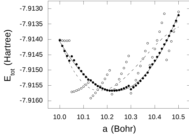
FIG. 5. Total energy of Si calculated at constant cut-off energy ( E_{cut}=6 Hartree with 2 special k -points in the IBZ) for 51 lattice constants. The open circles (o) represent the uncorrected values of total energy, whereas the solid circles (●) illustrate the values corrected by the S.H. technique. The solid curve and (resp.) the broken curve are obtained by a least-squares third-order fit to the corrected and (resp.) uncorrected data. The solid curve yields a lattice parameter of 10.23 Bohr, whereas the broken curve yields 10.17 Bohr.
