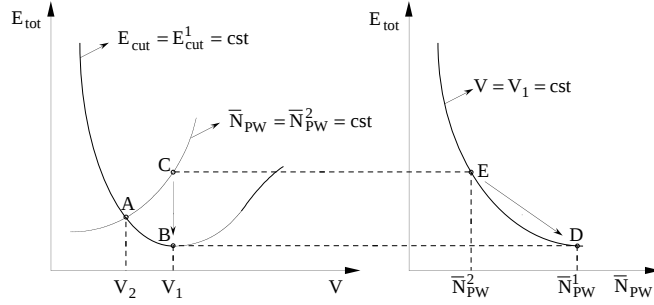
FIG. 3. Schematic representation of energy correction. The desired curve E_{tot}^c \{E_{cut}^1, V\} is the one going through points A and B. The calculated curve E_{tot}^d \{E_{cut}^1, V\} is the one going through points A and C. The correction at volume V_1 moves point C, obtained by a calculation with \bar{N}_{PW}^2 = \bar{N}_{PW}^d(E_{cut}^1, V_1) , to point B, obtained by an hypothetic calculation with \bar{N}_{PW}^1 = \bar{N}_{PW}^c(E_{cut}^1, V_1) . This operation is equivalent to moving point E to point D. This is easily done if the curve E_{tot}[\bar{N}_{PW}, V_1] is known (see Eq. (10)).
