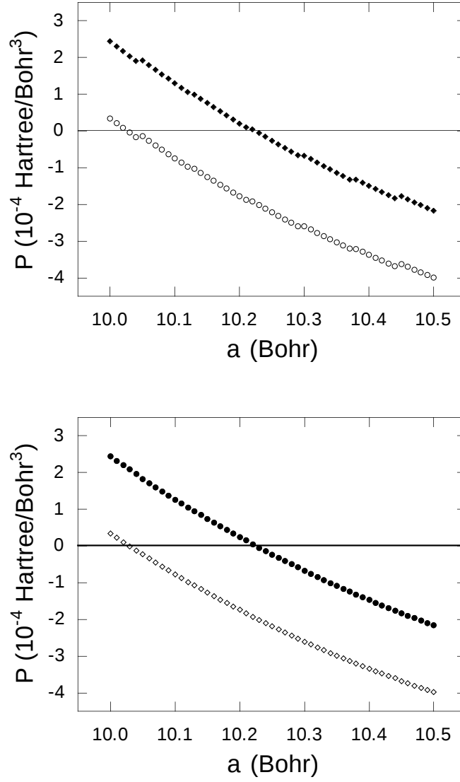
FIG. 4. Pressure in Si calculated at constant cut-off energy ( E_{cut}=6 Hartree with 2 special k -points in the IBZ) for 51 lattice constants. (a) The open circles ( \circ ) represent the uncorrected values of pressure, whereas the solid diamonds ( \blacklozenge ) illustrate the values corrected by the Froyen-Cohen technique. (b) The open diamonds ( \diamond ) represent partially corrected values of pressure (see P^* defined by Eq. (31) in the text), whereas the solid circles ( \bullet ) are the values corrected by the S.H. technique. The graphs (a) and (b) point out that the S.H. correction technique ( \bullet ) has two effects. The first is a shift of the uncorrected curve ( \circ ), also included in Froyen-Cohen technique ( \blacklozenge ). Whereas the second is the cancellation of micro-curve jumps present in the partial correction ( \diamond ).
