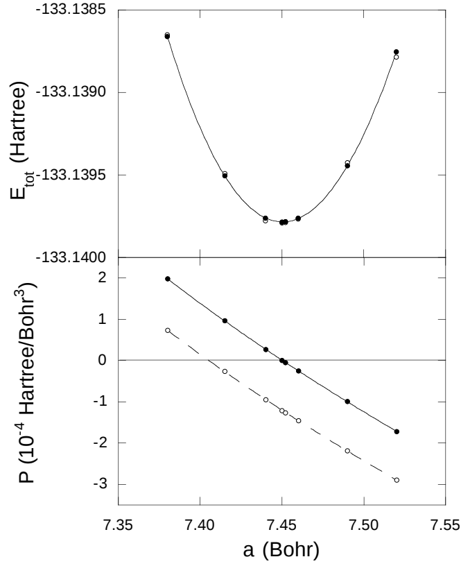
FIG. 7. Total energy and pressure of cubic BaTiO 3 calculated at constant cut-off energy ( E_{\text{cut}}=45 Hartree with 10 special k -points in the IBZ) for 8 lattice constants. The open circles ( \circ ) represent the uncorrected values (joined by a scattered dashed line), whereas the solid circles ( \bullet ) illustrate the values corrected by the S.H. technique. The corrected values of energy and pressure are joined by a least-squares third-order fit (solid curves). For total energy, the values obtained with or without correction are nearly the same (a high energy cut-off has been used, which leads to well converged values of total energy). For pressure, instead, the values obtained with or without correction differ despite the high energy cut-off. The lattice parameter value is found to be 7.45 Bohr from the solid lines.
