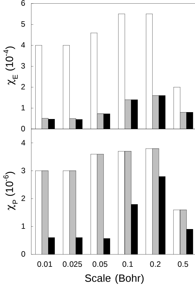
FIG. 9. Plot of standard deviations \chi_E (top) and \chi_P (bottom) of the energy and pressure data calculated at different scales at constant cut-off energy ( E_{cut}=6 Hartree with 2 special k -points in the IBZ) for 51 lattice constants. The white bars represent the standard deviation \chi calculated from uncorrected data, the gray bars illustrate the one calculated from the values corrected by Froyen-Cohen technique for pressure and by Francis-Payne technique for energy, whereas the black bars represent that calculated from the values corrected by the S.H. technique. The graph illustrates that the reduction of \chi is more important for small scales than large ones. Note also that Froyen-Cohen technique does not reduce the noise in the pressure data.
