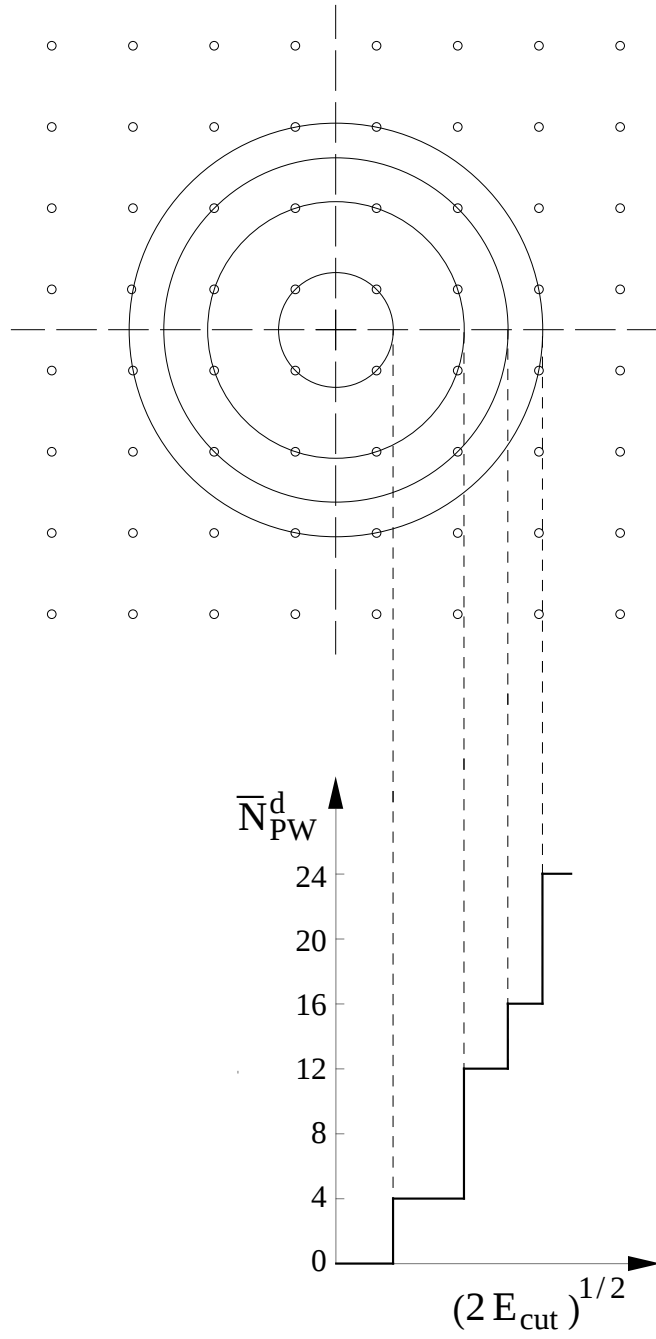
FIG. 1. Number of plane waves \bar{N}_{PW}^d in a basis set defined by Eq. (2) in a 2D case. The upper graph illustrates how these k-points are enclosed in a circle of radius (2E_{cut})^{1/2} . The lower graph illustrates the stair-like evolution of \bar{N}_{PW}^d as a function of E_{cut} .
