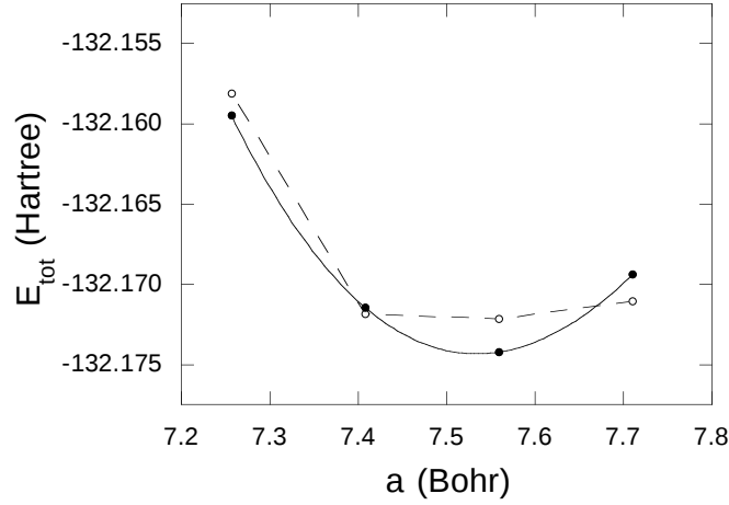
FIG. 6. Total energy of cubic BaTiO 3 calculated at constant cut-off energy ( E_{cut}=20 Hartree with 4 special k -points in the IBZ) for 4 lattice constants. The open circles (o) represent the uncorrected values of total energy, whereas the solid circles (●) are the values corrected by the S.H. technique. The corrected values of energy are joined by a least-squares third-order fit (solid curve). Without correction, the residual noise leads to incorrect values of the static equilibrium properties, as there are not enough data. The lattice parameter value is found to be 7.53 Bohr from the solid line.
