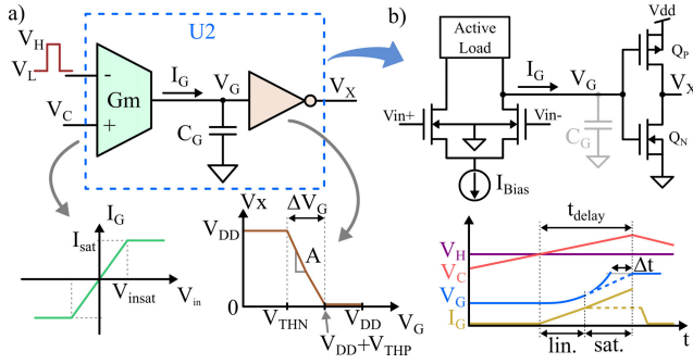
Fig. 3. (a) Block diagram of the comparator with the transfer function of each device. V_{THN} and V_{THP} are the threshold voltages of nMOS and pMOS transistors, respectively. (b) Schematic of a generic comparator and time-domain signals at different nodes.
