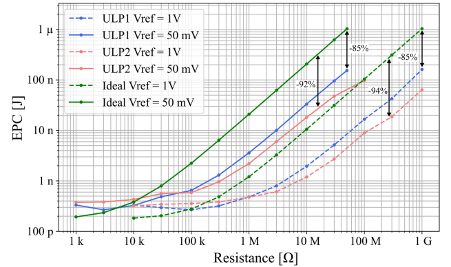
Fig. 13. Measured EPC for ULP1 and ULP2 compared to an ideal readout interface whose comparators are biased with 3 μA dc each.
