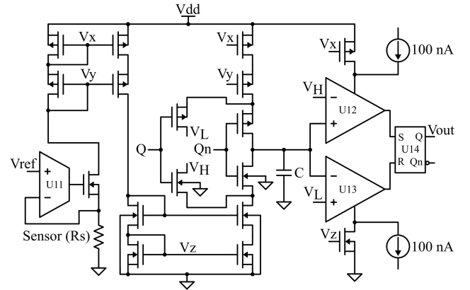
Fig. 9. Schematic of readout ULP2, the comparators are biased with a fixed 100 nA plus a reduced copy of the current through the sensor.
