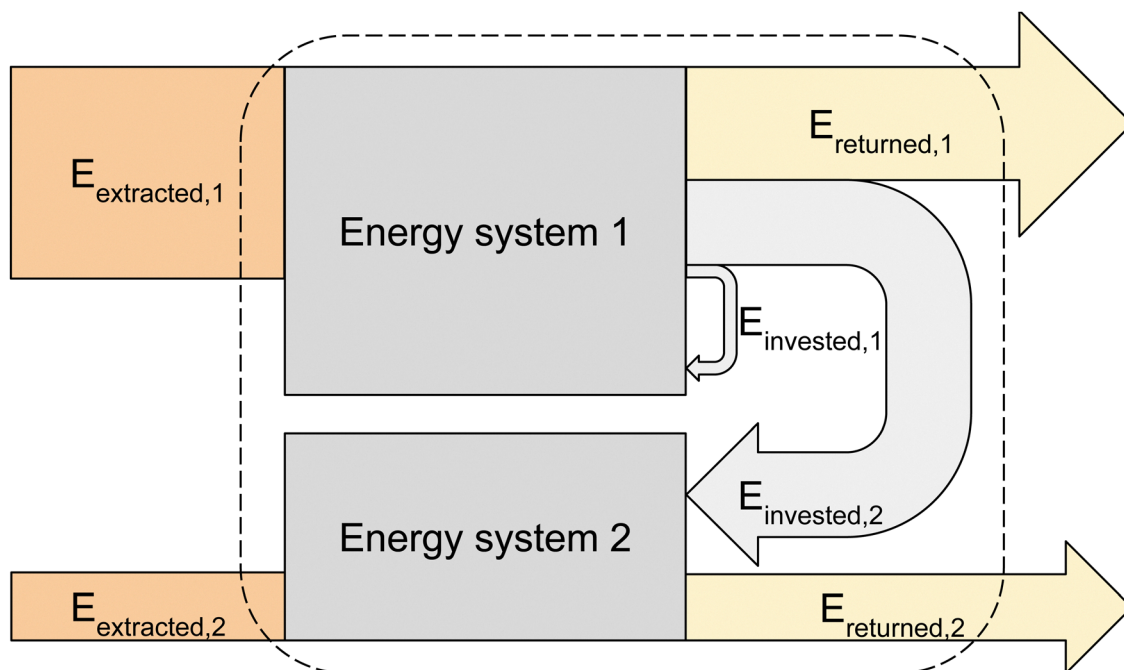
Fig. 1 Returned energy as a function of the extracted and the invested energy for two systems. EROI (global) = (E_{\text{returned},1} + E_{\text{returned},2}) / (E_{\text{invested},1} + E_{\text{invested},2}) . EROI (energy system 2) = E_{\text{returned},2} / E_{\text{invested},2} . Energy losses are omitted for clarity.
