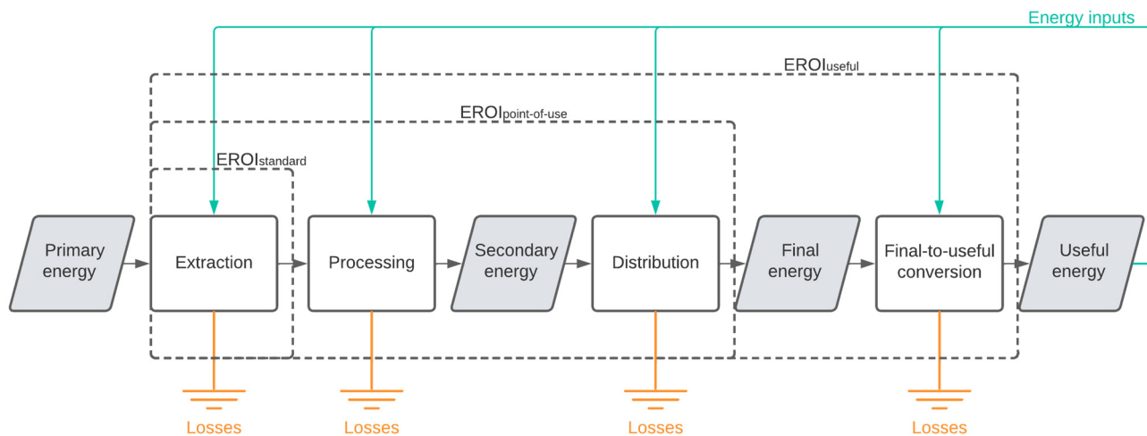
Fig. 2 Standard, or primary stage EROI ( EROI_{\text{standard}} ), point-of-use or final stage EROI ( EROI_{\text{point-of-use}} ) and useful EROI ( EROI_{\text{useful}} ).
