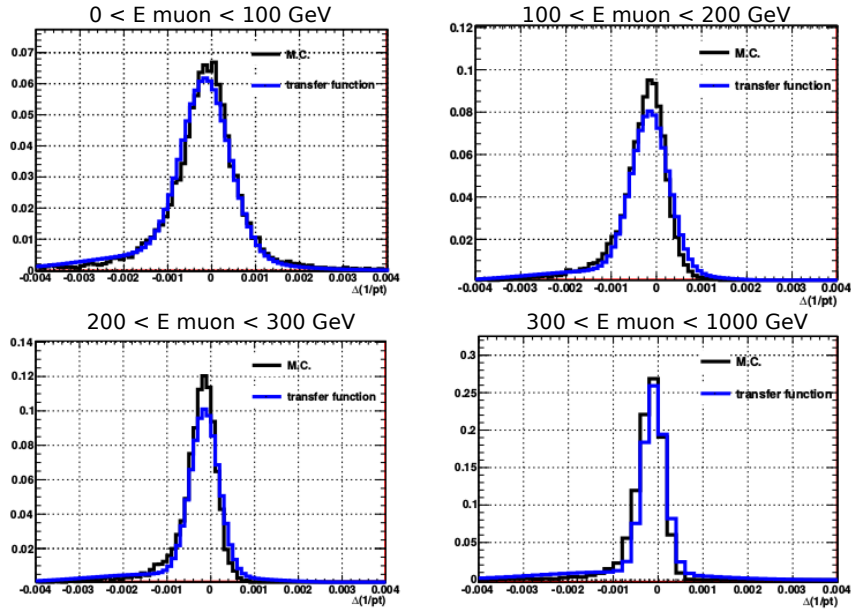
Figure 2.17: Comparison of the TF obtained for muons, with the expected \Delta \frac{1}{p_T} = \left( \frac{1}{p_T} \right) - \left( \frac{1}{p_T} \right)^{\text{vis}} distribution, for different generated muon energy ranges.
