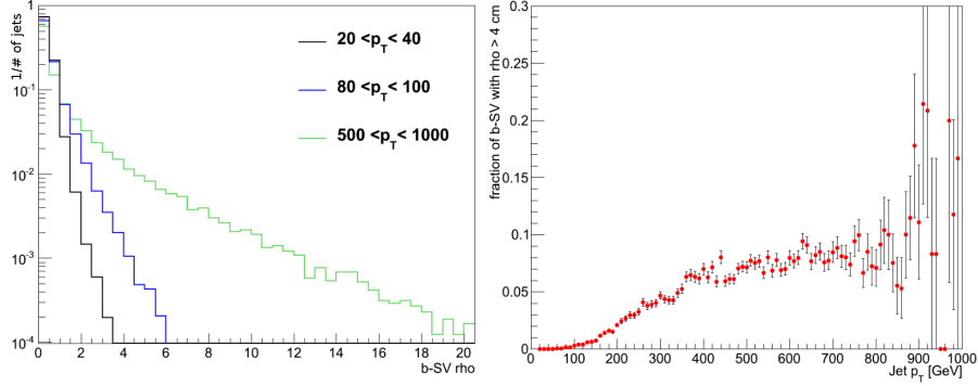
Figure 3.22: Left: distribution of the flying distance of the B hadron in the \rho plane for different jet p_T . Right: fraction of B hadrons when \rho > 4 \text{ cm} , as a function of jet p_T .
