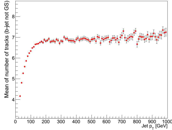
Figure 3.14: Multiplicity of reconstructed tracks inside a b jet, as a function of the jet p_T .
