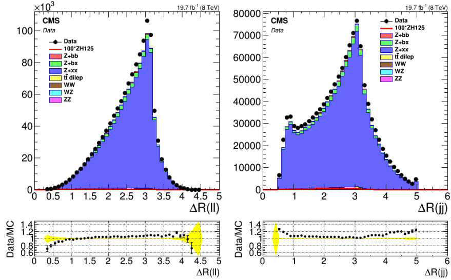
Figure C.14: Distributions of the \Delta R(ll) and \Delta R(jj) (right), at "ll+jj+X" stage, with a FR like selection.
