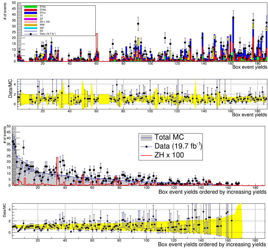
Figure 5.17: Distribution of the final discriminant used for the exclusion limit on the ZH strength determination, for the light-like 3-jets boxes, for all the different processes and the data (top), and for the sum of all the MC processes versus the data ordered by expected event yields (bottom). The yellow bands represent the statistical uncertainty on the MC distributions.
