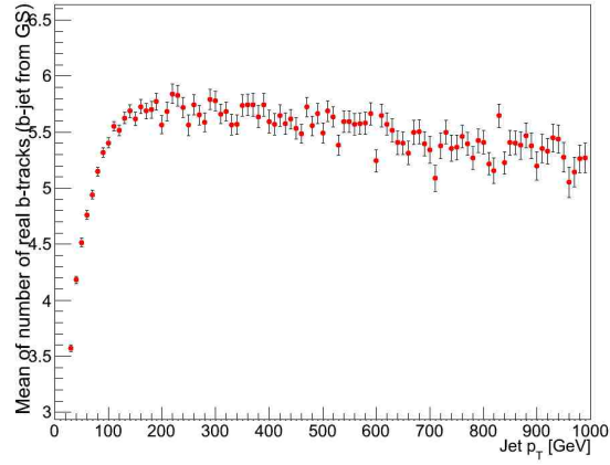
Figure 3.19: Multiplicity of tracks real B tracks from GS jets, as a function of the jet p_T , inside a b jet.
