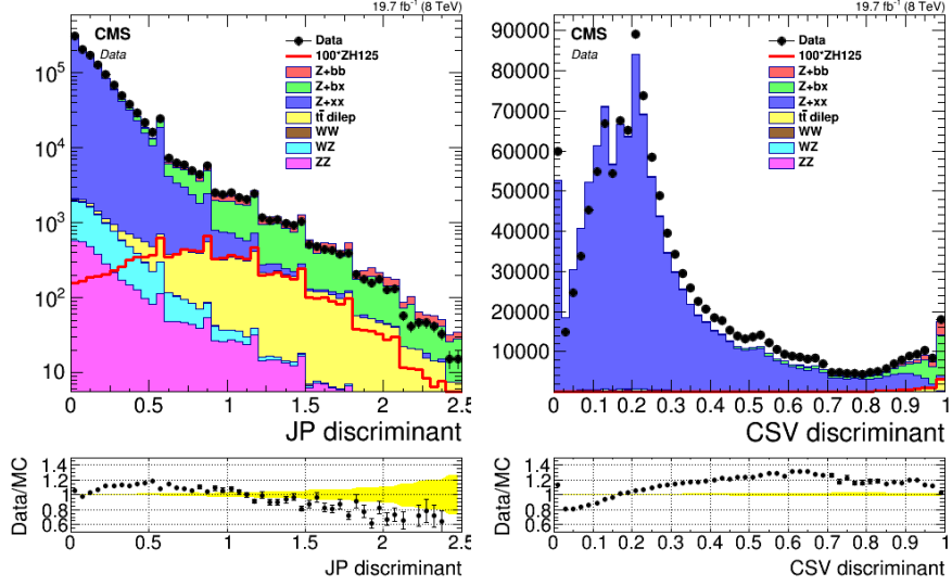
Figure 4.15: Distributions of the JP discriminator (left), and of the CSV discriminator (right), at “ ll+jj+X ” stage. The FR selection has been applied, except for the b -tagging requirement and the MET cut.
