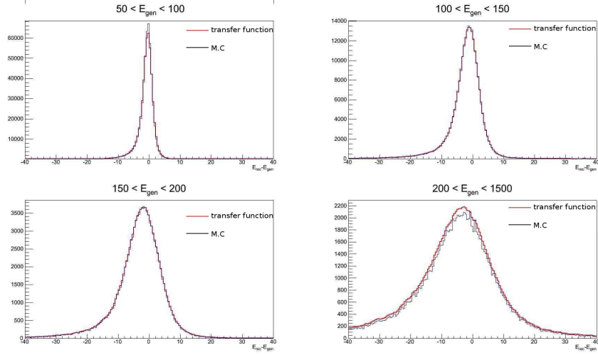
Figure A.4: Comparison of the TF obtained for muons, with the expected \Delta E = E - E^{\text{vis}} distribution, for different generated muon energy ranges.
