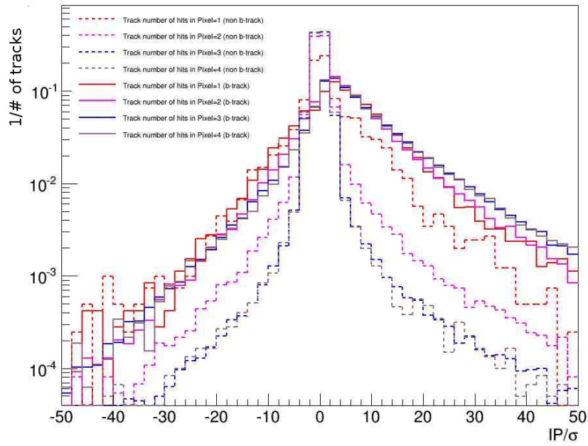
Figure B.8: Distribution of the IP/\sigma for tracks with different number of hits in the pixel detector, for B tracks (solid lines) and non B tracks (dashed lines).
