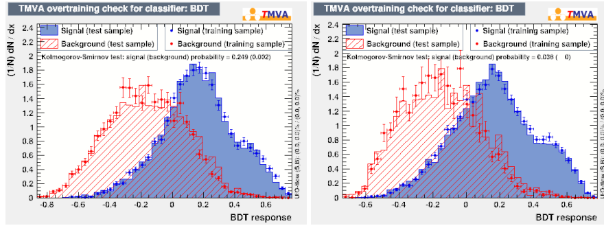
Figure C.50: TMVA BDT output ZH versus all backgrounds, for the 2-jets (left) and 3-jets (right) categories.
