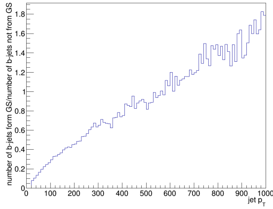
Figure 3.18: Ratio of the number of b jets coming from GS over the number of b jets not coming from GS, as a function of the jet p_T .
