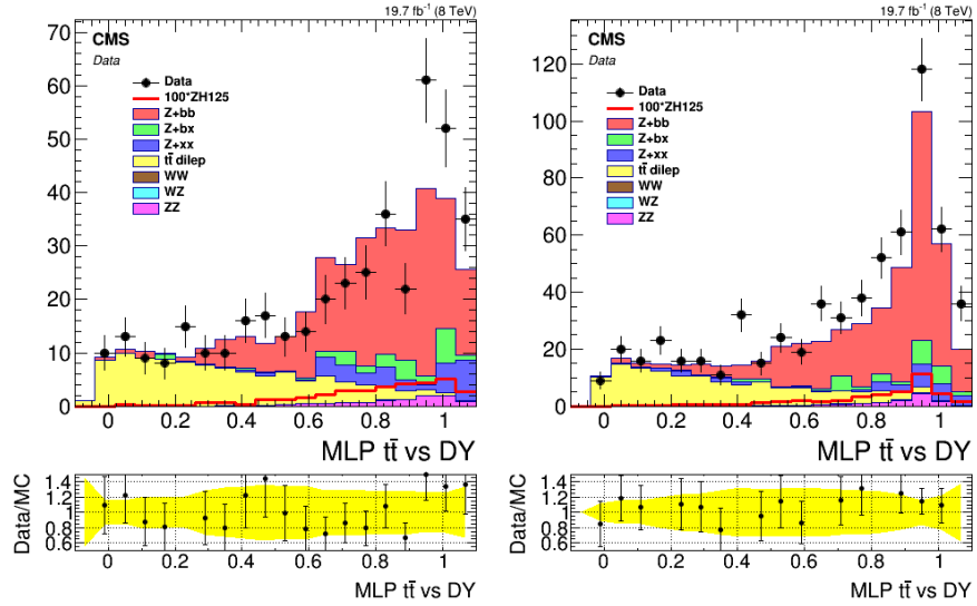
Figure 4.12: Neural-Net output used to discriminate DY events from t\bar{t} events, in the CR. Left plots represent the di-electron channel, right plots the di-muon channel, for the 2-jets category.
