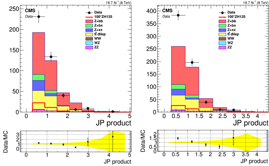
Figure 4.10: Product of the two leading b jets JP discriminator values, used to discriminate b jets from light jets contributions, in the CR. The left plot is in the di-electron channel and the right plot in the di-muon channel, for the 2-jets category.
