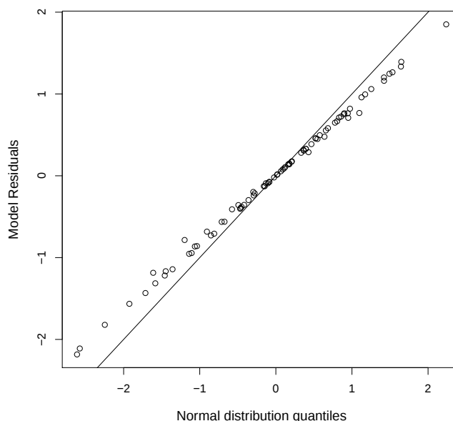
Figure 10. Normal probability distribution of model residuals for the predicted log transformed mean nitrate concentration.
