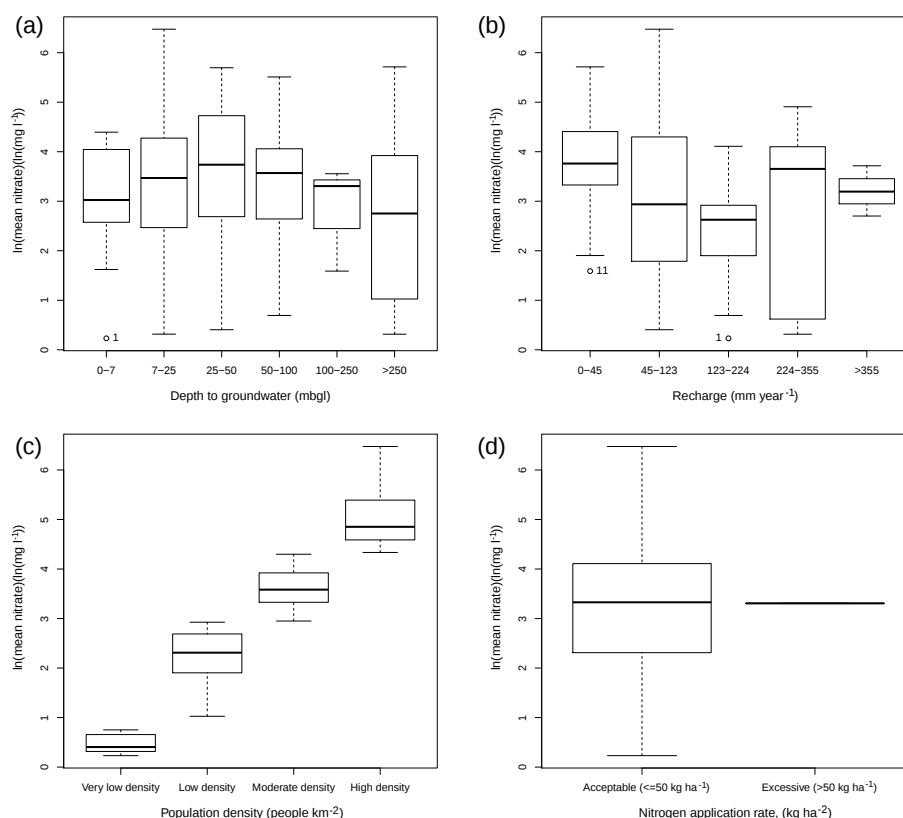
Figure 8. Log transformed mean nitrate concentration for different groundwater depth classes (a), recharge classes (b), population density classes (c) and nitrogen application rate classes (d).
