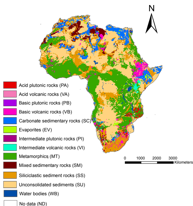
Figure 1. Hydrogeological setting of the African continent (from Hartmann and Moosdorf, 2012).
