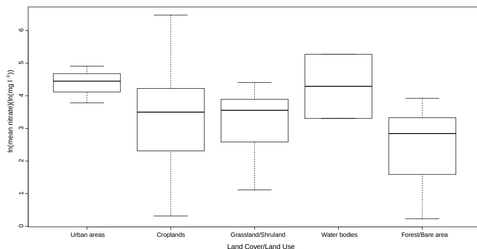
Figure 6. Log transformed mean nitrate concentration for different land use classes.
