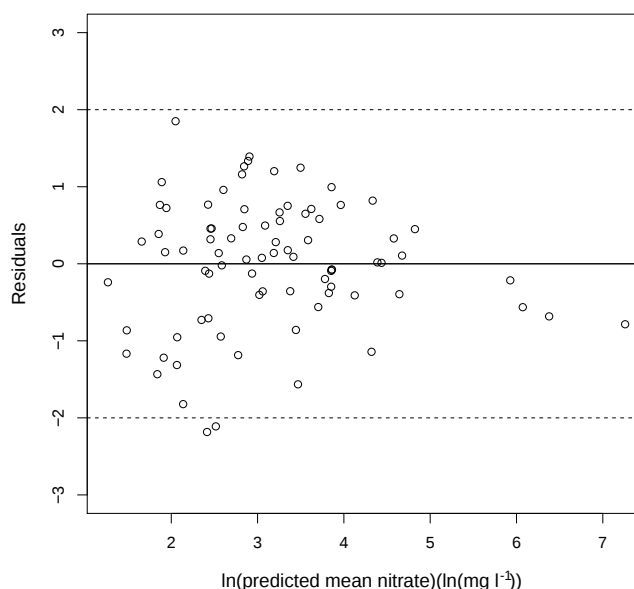
Figure 11. Relation between residuals and predicted log transformed mean nitrate concentration.
