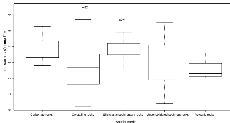
Figure 7. Log transformed mean nitrate concentration for different aquifer system classes.
