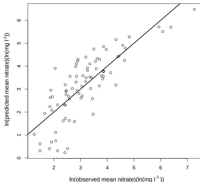
Figure 9. Predicted vs. observed mean log transformed nitrate concentration ( R^2 = 0.65 ).
