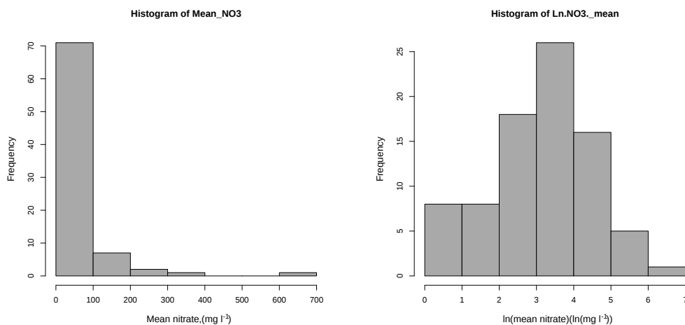
Figure 5. Histograms of observed mean nitrate concentration ( \text{mg L}^{-1} ) and log transformed mean nitrate concentration ( \ln(\text{mg L}^{-1}) ).
