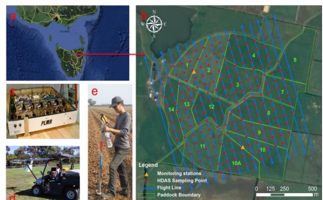
Figure 1. (a) Location of the study area in Tasmania Australia; (b) Flight lines and sampling points; (c) the Polarmetric L-band Multibeam Radiometer (PLMR) system; (d) the ESA L-band radiometer (ELBARA III); and (e) the Hydraprobe Data Acquisition System (HDAS) used for ground truthing.
