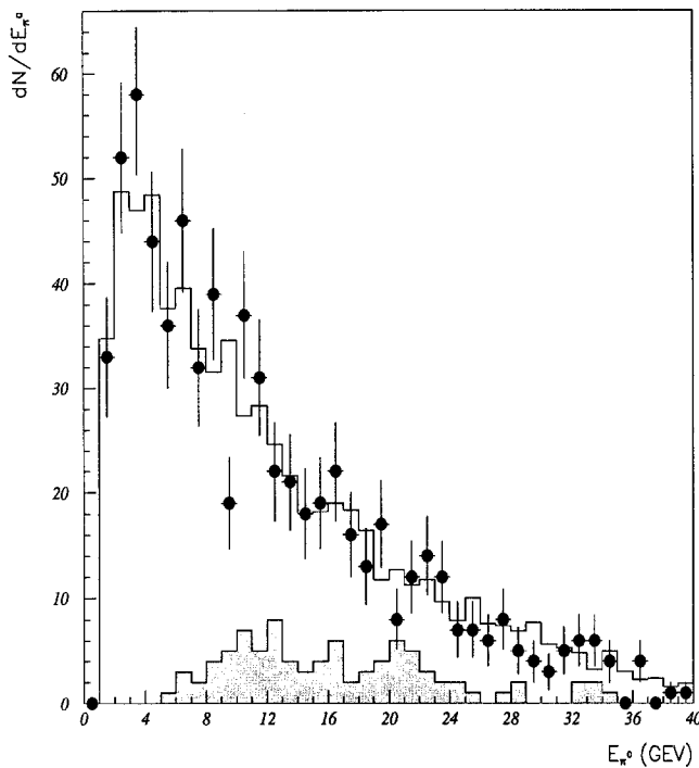
Fig. 7. Energy of the neutral particle produced in the decay \tau^- \rightarrow \rho^- \nu_\tau , \rho^- \rightarrow \pi\pi^0 for data (points with error bars) and Monte Carlo simulation (solid line); the shaded area corresponds to the contribution of the energetic \pi^0 (the two photons are not resolved into two neutrals but identified using the first three layers of the HPC)
