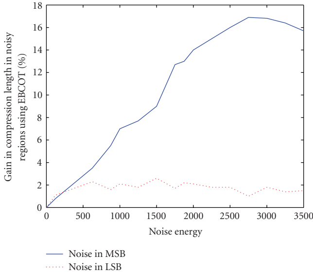
FIGURE 18: Spatial modeling increases the system performances when the reference available at the client is erroneous. This figure illustrates the increase in compression efficiency brought by the spatial modeler when noise is added to the reference LSB and MSB bit-planes. These results have been generated using code-blocks of the third resolution of the Speedway sequence.
