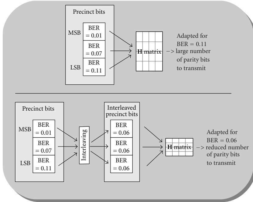
FIGURE 10: Precinct layer bit-planes interleaving. When multiple codewords are generated for a given precinct, interleaving of the bits enables to make the distribution of errors uniform and consequently reduces the size of the matrix \mathbf{H} required to correct the precinct, reducing the number of parity bits to transmit.
