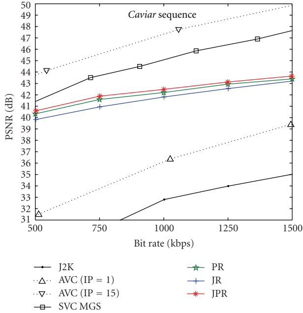
FIGURE 16: Performances of the proposed system with different combination of Parity and JPEG 2000 replenishments (JR, PR, and JPR), MPEG4-AVC), and the purely INTRA JPEG 2000 coding scheme (J2K) for the Caviar sequence.
