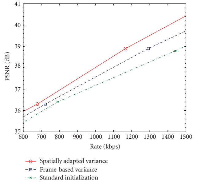
FIGURE 17: Comparison of the three methods exploiting the temporal correlation between frames in the wavelet domain.
