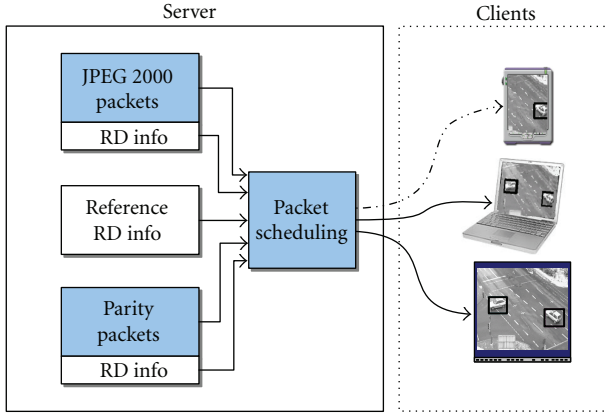
FIGURE 1: Proposed system architecture. Based on a rate-distortion analysis, the server decides for each precinct either to transmit the corresponding JPEG 2000 packet, to forward a parity packet, or to recommend the use of the available reference to the client. The scheduler takes these decisions at transmission time independently for each user based on its individual requests of interest and available resources.
