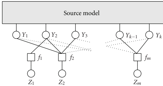
FIGURE 5: Factor graph representing the source model and the LDPC code. At each iteration of the decoding process, messages describing local distributions are exchanged between nodes inside the LDPC code and with the source model.
