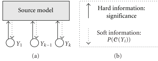
FIGURE 9: Hard decisions are transmitted from each LDPC node, and soft information calculated in the Source Modeler is sent back.
