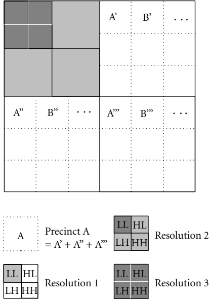
FIGURE 3: JPEG 2000 wavelet subbands and precincts. A first discrete wavelet transform is applied on the original image, generating four subbands . The DWT is then applied recursively on the LL subbands containing the low frequencies of each resolution. A precinct is a spatial subdivision of a resolution and corresponds to the same spatial zones in each subband.
