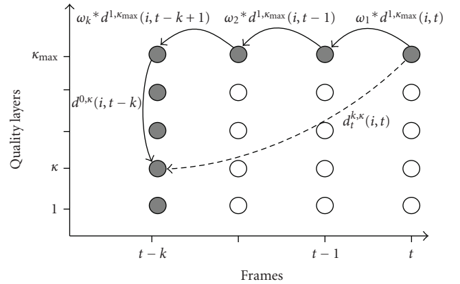
FIGURE 13: Path used to approximate the distortion of the previous references, compared to the optimal path (dashed arrow). This approximation significantly decreases the pre-processing complexity and storage requirements, without significantly impairing the streaming performance.
