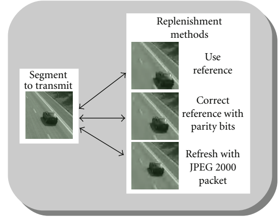
FIGURE 2: Given an image segment to transmit, the system recommends the client to use one of the 3 available replenishment options, depending on rate-distortion analysis.
