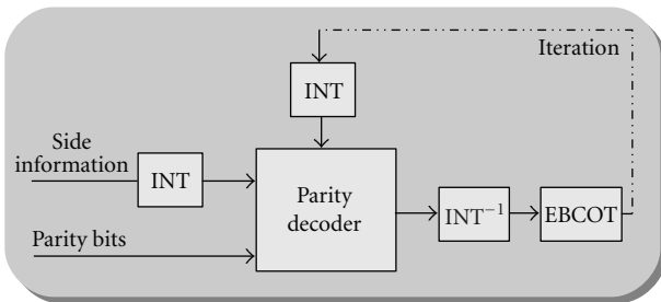
FIGURE 11: Interleaving operations at decoding. To decode a precinct, an interleaved (INT) version of the side information and the corresponding received parity bits are fed to the parity decoder. At each iteration of the sum-product algorithm, the hard decisions of each bit are deinterleaved ( \text{INT}^{-1} ) and transmitted to the EBCOT. The EBCOT output, consisting in soft information for each bit, is interleaved and fed into the parity decoder for the next iteration.
