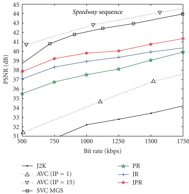
FIGURE 15: Performances of the proposed system with different combination of Parity and JPEG 2000 replenishments (JR, PR, and JPR), MPEG4-AVC), and the purely INTRA JPEG 2000 coding scheme (J2K) for the Speedway sequence. Frame rates and encoding parameters are defined in the text.
