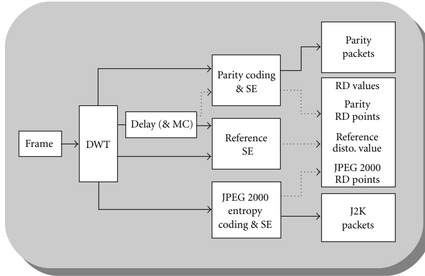
FIGURE 14: Generation of compressed data and rate-distortion information at the encoder side. The main modules consist in the discrete wavelet transform, the delay (and optional motion compensation) module, the generation of Parity, and JPEG 2000 data with its associated squared error (SE) and the calculation of the reference squared error.
