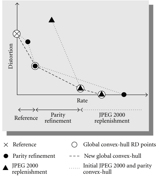
FIGURE 12: Rate-distortion representation of the replenishment decisions for a given precinct. Depending on the available bit-rate, the client will use the reference (cross) and receive a parity packet (dot) or JPEG 2000 packets (triangles). The original JPEG 2000 RD points and the resulting replenishment decisions lie on convex-hulls.
