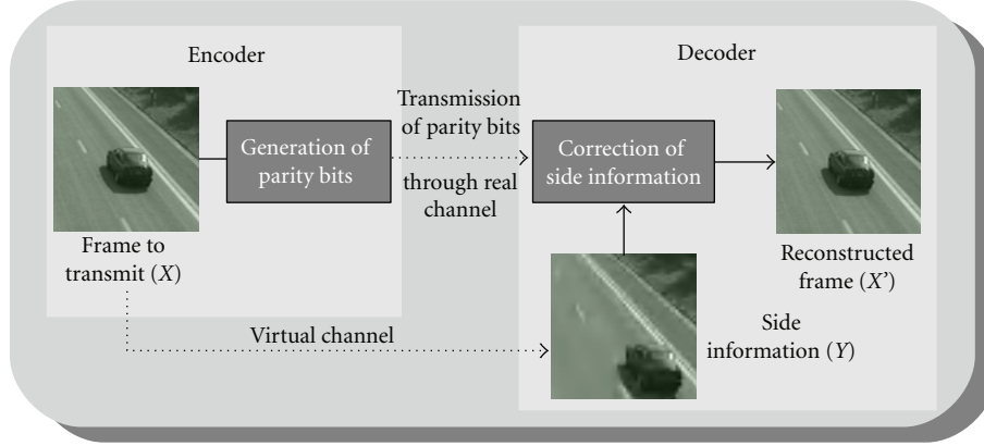
FIGURE 4: Video coding system with side information. Parity bits are generated at the encoder based on the frame to transmit. With these parity bits, the decoder corrects the side information, which is usually the previous decoded frame, and generates the reconstructed frame.
