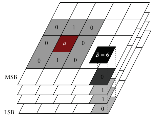
FIGURE 8: Bit-plane representation. The coefficient B which is equal to 6 is represented in binary form (0110) through the four bit-planes. Its MSB is insignificant, and the remaining bits of the coefficient are significant. Bit-plane context modeling. The context of bit a is calculated based on its eight neighbors significance as well as its own significance state.
