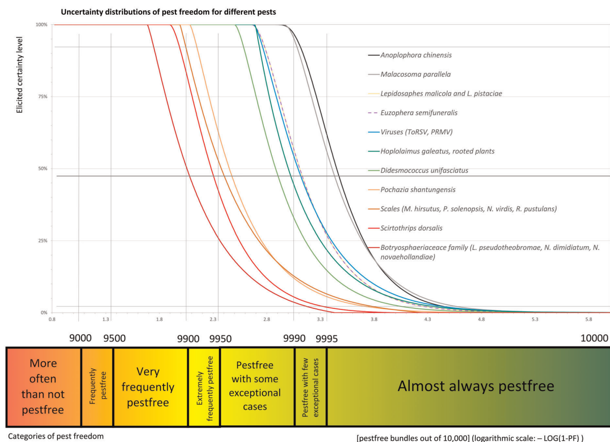
Figure 6: Elicited certainty (y-axis) of the number of pest-free Prunus persica and P. dulcis , as budwood/graftwood, bare-rooted or grafted on rootstocks of either P. persica , P. dulcis , P. armeniaca , P. davidiana or their hybrids bundles (x-axis; log-scaled) out of 10,000 plants designated for export to the EU from Türkiye for all evaluated pests visualised as descending distribution function. Horizontal lines indicate the percentiles (starting from the bottom 5%, 25%, 50%, 75%, 95%). The Panel is 95% confident that 9,992, 9,991, 9,982, 9,982, 9,982, 9,973, 9,926, 9,906, 9,891, 9,813 or more bundles per 10,000 will be free from A. chinensis , M. parallela , Lepidosaphes group ( L. malicola and L. pistaciae ), E. semifuneralis , Viruses (PRMV and ToRSV), H. galeatus , D. unifasciatus , P. shantungensis , scales ( M. hirsutus , N. viridis , P. solenopsis , R. pustulans , S. dorsalis ), Botryosphaeriaceae family ( L. pseudotheobromae , N. dimidiatum , N. novaehollandiae ), respectively
