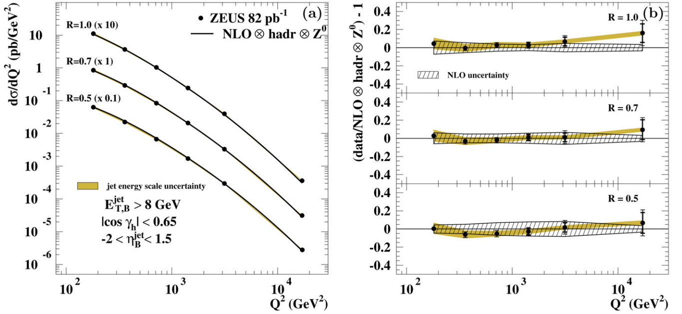
Fig. 2. The measured differential cross section d\sigma/dQ^2 for inclusive-jet production with E_{T,B}^{\text{jet}} > 8 GeV and -2 < \eta_B^{\text{jet}} < 1.5 (dots) for different jet radii, in the kinematic range given by |\cos \gamma_h| < 0.65 . Other details as in the caption to Fig. 1.
