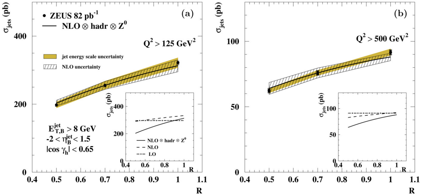
Fig. 3. The measured cross section \sigma_{\text{jets}} as a function of the jet radius for inclusive-jet production with E_{T,B}^{\text{jet}} > 8 GeV and -2 < \eta_B^{\text{jet}} < 1.5 (dots), in the kinematic range given by |\cos \gamma_h| < 0.65 and (a) Q^2 > 125 GeV 2 and (b) Q^2 > 500 GeV 2 . The insets show the LO (dot-dashed lines) and NLO (dashed lines) QCD calculations. The NLO QCD calculations corrected to include hadronisation and Z 0 effects are shown as solid lines. Other details as in the caption to Fig. 1.
