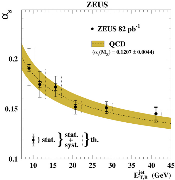
Fig. 4. The \alpha_s values determined from the measured d\sigma/dE_{T,B}^{\text{jet}} with R = 1 as a function of E_{T,B}^{\text{jet}} (dots). The dashed line indicates the renormalisation group prediction at two loops obtained from the \alpha_s(M_Z) value determined in this analysis and the shaded area represents its uncertainty. The inner error bars represent the statistical uncertainties of the data. The outer error bars show the statistical and systematic uncertainties added in quadrature. The dotted vertical bars, shifted to aid visibility, represent the theoretical uncertainties.
