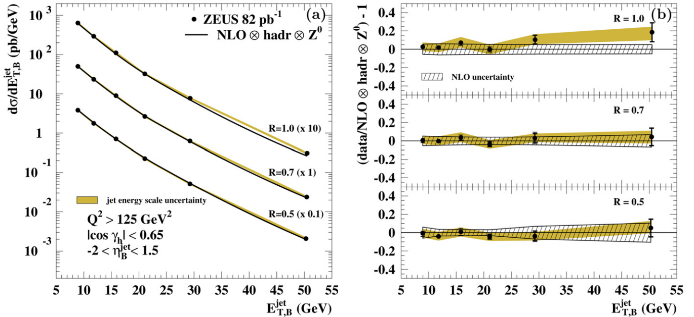
Fig. 1. (a) The measured differential cross section d\sigma/dE_{T,B}^{\text{jet}} for inclusive-jet production with -2 < \eta_B^{\text{jet}} < 1.5 (dots) for different jet radii, in the kinematic range given by Q^2 > 125 \text{ GeV}^2 and |\cos \gamma_h| < 0.65 . The NLO QCD calculations with \mu_R = E_{T,B}^{\text{jet}} (solid lines), corrected to include hadronisation and Z^0 effects and using the ZEUS-S parameterisations of the proton PDFs, are also shown. Each cross section has been multiplied by the scale factor indicated in brackets to aid visibility. (b) The fractional differences between the measured d\sigma/dE_{T,B}^{\text{jet}} and the NLO QCD calculations (dots); the hatched bands display the total theoretical uncertainty. The inner error bars represent the statistical uncertainty. The outer error bars show the statistical and systematic uncertainties, not associated with the uncertainty in the absolute energy scale of the jets, added in quadrature. The shaded bands display the uncertainty due to the absolute energy scale of the jets.
