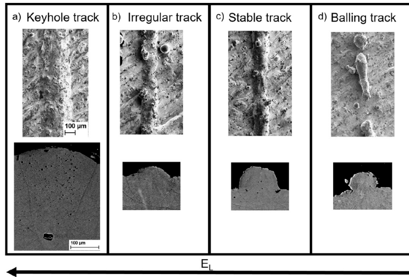
Fig. 5. SEM images of the top views and cross sections of the four types of SST in function of E_L . The L-PBF parameters are a) P = 273 W and v = 600 mm/s, b) P = 218 W and v = 1300 mm/s, c) P = 218 W and v = 1600 mm/s and d) P = 164 W and v = 2400 mm/s.
