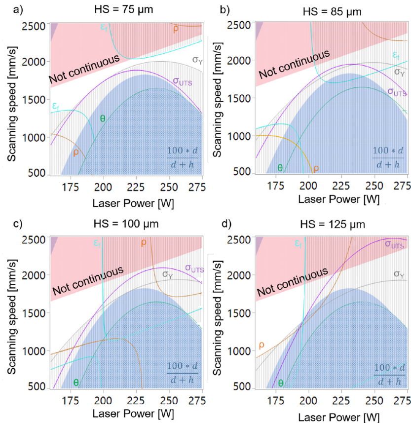
Fig. 10. Process window obtained based on all the models developed with the proposed methodology (SST, density and tensile mechanical properties) in function of P and v for a) HS = 75 \mu m , b) HS = 85 \mu m , c) HS = 100 \mu m and d) HS = 125 \mu m . The white area is the process window, while the dashed area is the zone which does not fulfill the desirability criteria for the mechanical properties and the density. The red, blue and dotted area corresponds to the parameters leading to non continuous tracks and inadequate 100 \cdot d / (d + h) and contact angle, respectively. (For interpretation of the references to color in this figure legend, the reader is referred to the web version of this article.)
