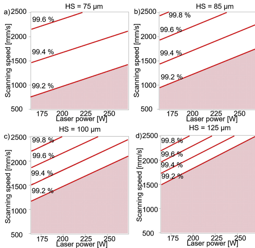
Fig. 9. Density of cubes measured by Archimedes density method for a) HS = 75 \mu\text{m} , b) HS = 85 \mu\text{m} , c) HS = 100 \mu\text{m} and d) HS = 125 \mu\text{m} . The red area contains the L-PBF parameters leading to density smaller than 99.2%. The red lines are iso-responses i.e. constant density. (For interpretation of the references to color in this figure legend, the reader is referred to the web version of this article.)
