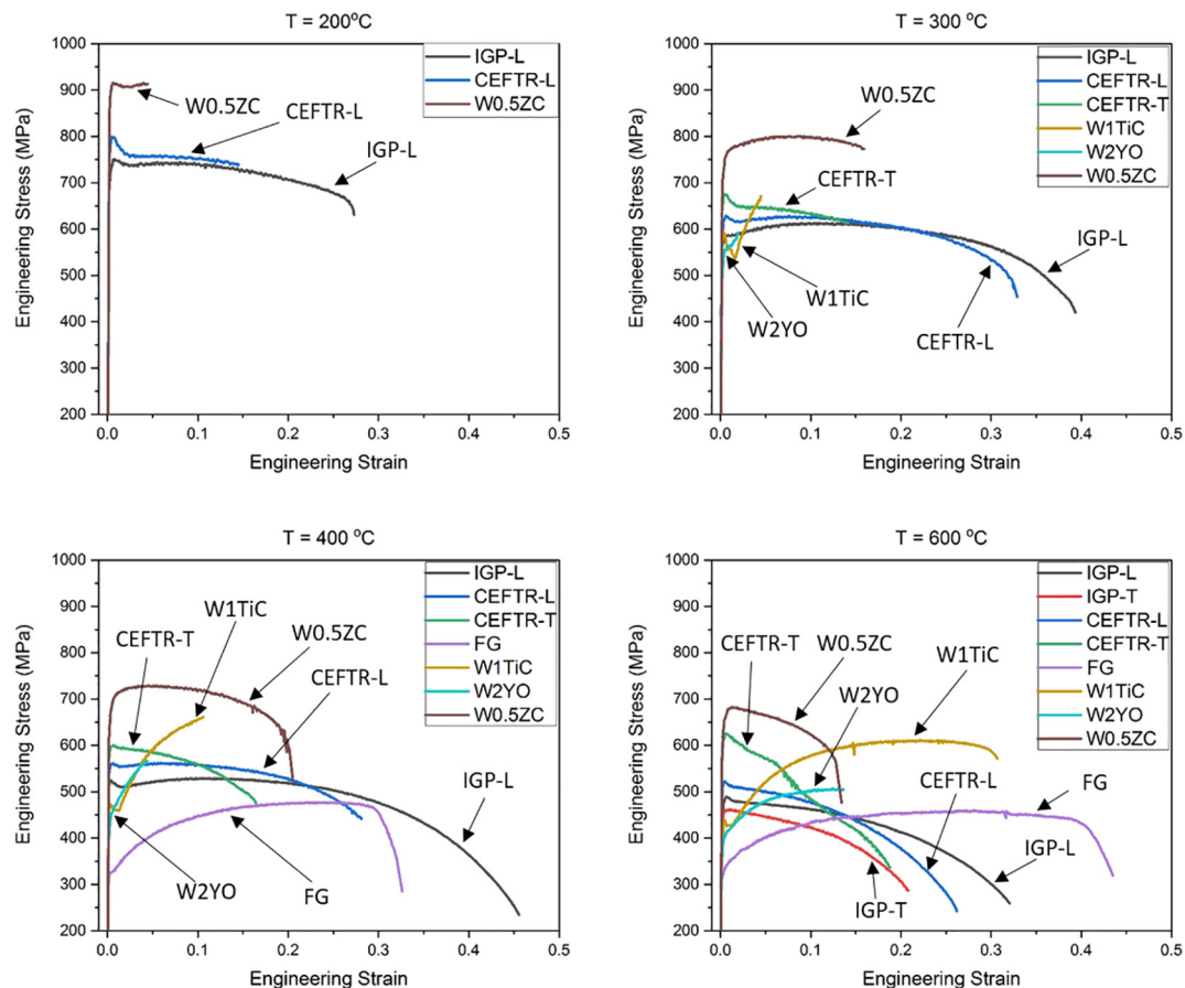
Fig. 4. Stress-strain curve of baseline and advanced W.
