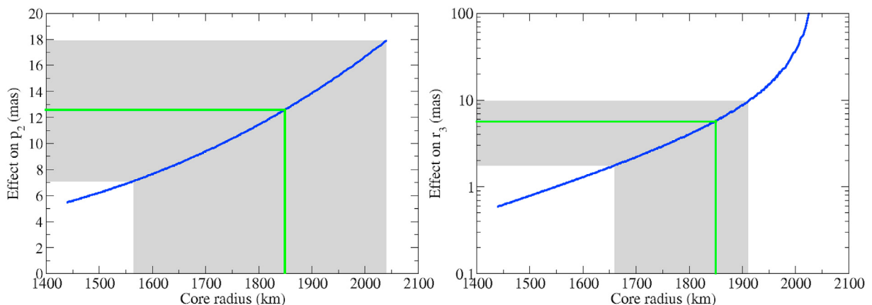
Fig. 8. Amplification of the p_2 and r_3 because of the liquid core as a function of core radius and link between the nutation uncertainty and core radius uncertainty. The elastic hydrostatic models with the EH45 Mars mantle mineralogy and a hot mantle end-member temperature profile are considered. A liquid convecting Fe-S core is assumed. The grey region illustrates the nominal case for an average core size r_{cmb} = 1850 km.
