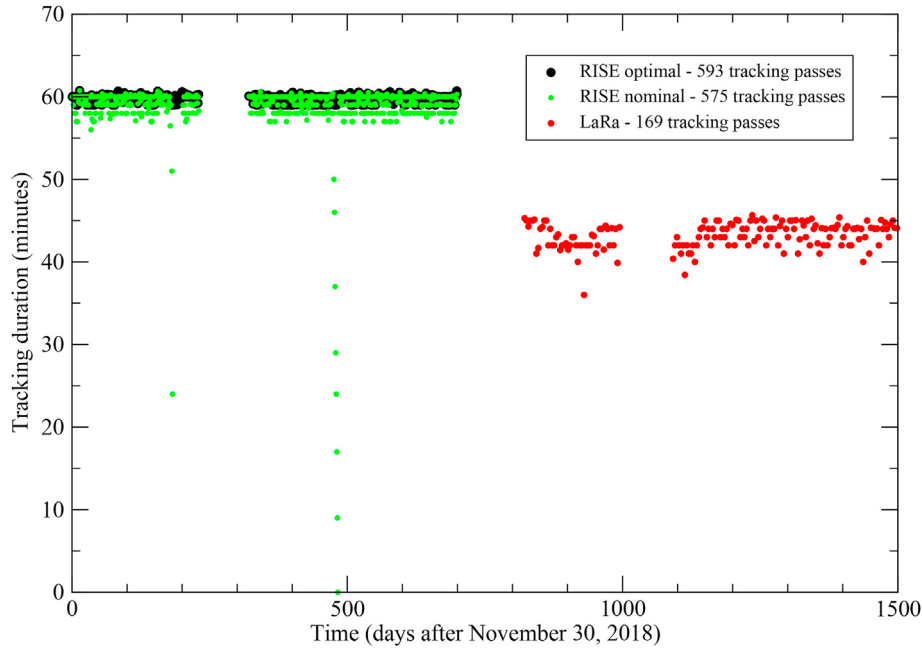
Fig. 4. Temporal evolution of the tracking duration for LaRa, RISE optimal and RISE nominal.
