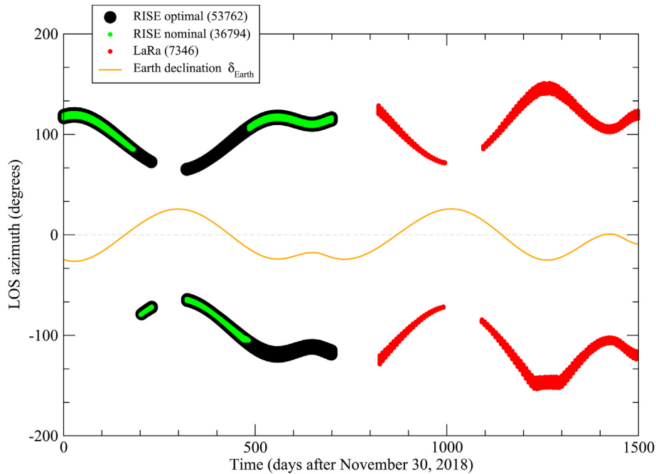
Fig. 2. Temporal evolution of Earth LOS azimuth for both transponders. LaRa is in red, RISE optimal case is in black and RISE nominal case is in green. The orange line shows the Earth declination \delta_{Earth} (in degrees). The number of data points is indicated in brackets. (For interpretation of the references to colour in this figure legend, the reader is referred to the Web version of this article.)
