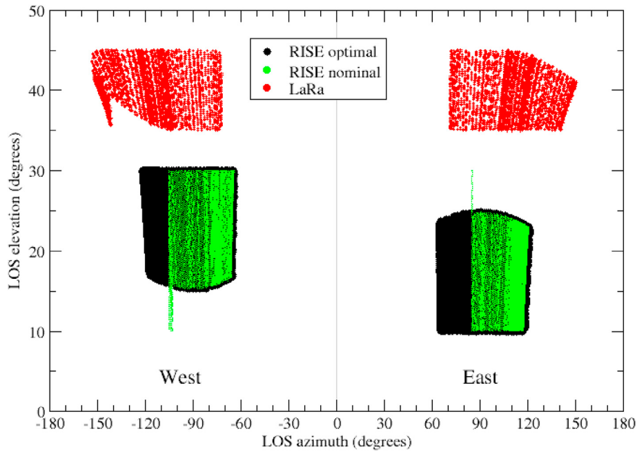
Fig. 1. Earth LOS direction in terms of azimuth and elevation for both transponders. LaRa is in red and the different RISE configurations are the optimal case in black and the nominal case in green. (For interpretation of the references to colour in this figure legend, the reader is referred to the Web version of this article.)
