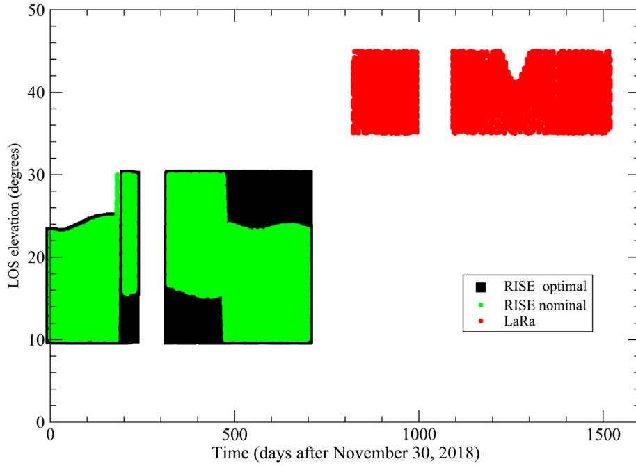
Fig. 3. Temporal evolution of Earth LOS elevation for both transponders. LaRa is in red, RISE optimal case is in black and RISE nominal case is in green. (For interpretation of the references to colour in this figure legend, the reader is referred to the Web version of this article.)
