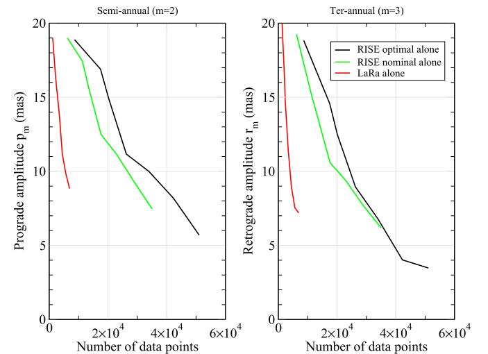
Fig. 5. Uncertainty ( 1\sigma ) on p_2 and r_3 as a function of data points for the optimal and nominal RISE configurations and for the nominal LaRa configuration. The amplitudes are expressed in milliarcseconds (mas). 1 mas corresponds to 1.6 cm on Mars' surface.
