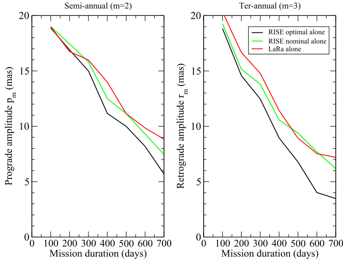
Fig. 6. Temporal evolution of the nutation uncertainties as estimated by RISE optimal case (in black), RISE nominal case (in green) and LaRa (in red) separately. (For interpretation of the references to colour in this figure legend, the reader is referred to the Web version of this article.)
