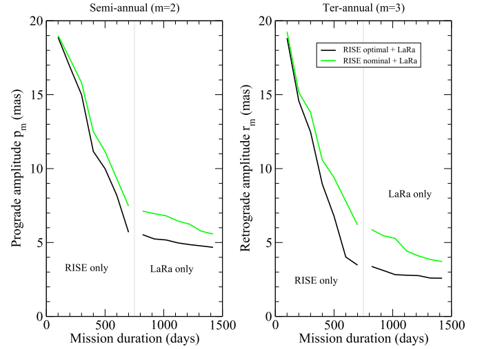
Fig. 7. Effect of combining RISE and LaRa on the p_2 and r_3 nutation uncertainties for the nominal RISE optimal case and the RISE nominal case followed by LaRa.
