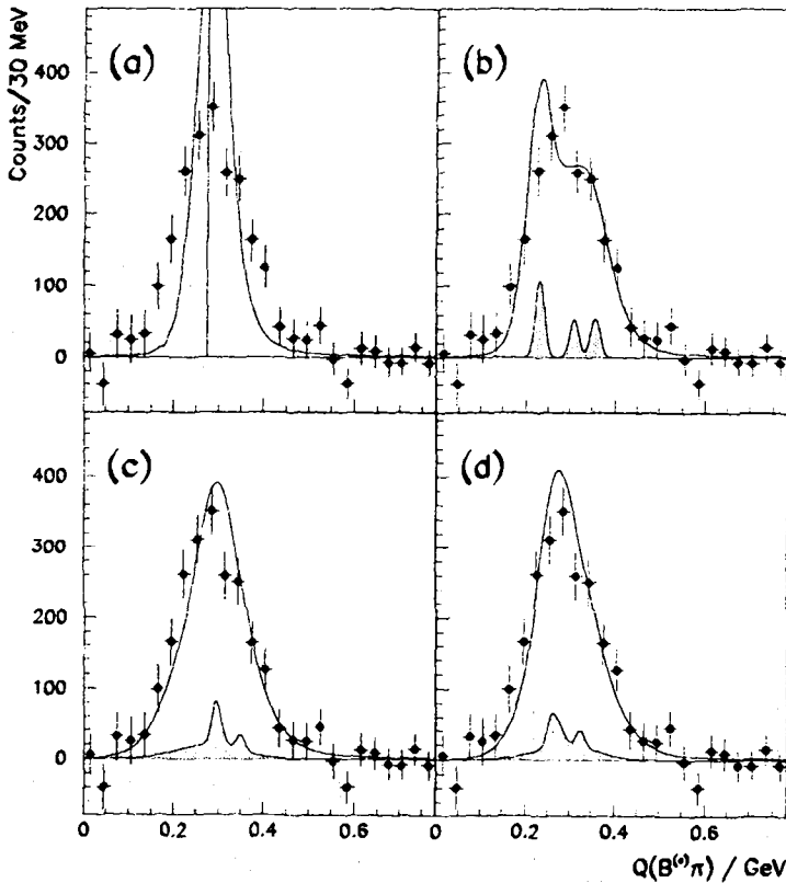
Fig. 2. Comparison of the background subtracted Q-value distribution (data points) with various models (solid line). The shaded area corresponds to the generated distribution (scaled by a factor 0.2) prior to detector resolution effects : (a) a delta-function at Q = 284 \text{ MeV}/c^2 (detector resolution including non-Gaussian tails). (b) two narrow resonances, one decaying into B\pi , the other equally into B\pi and B^*\pi . A mass splitting of 80 \text{ MeV}/c^2 is necessary to describe the observed width. (c) the model of Eichten et al. [18], plus broad resonances shifted downwards by 50 \text{ MeV}/c^2 . (d) two narrow and two broad states without large mass splitting.
