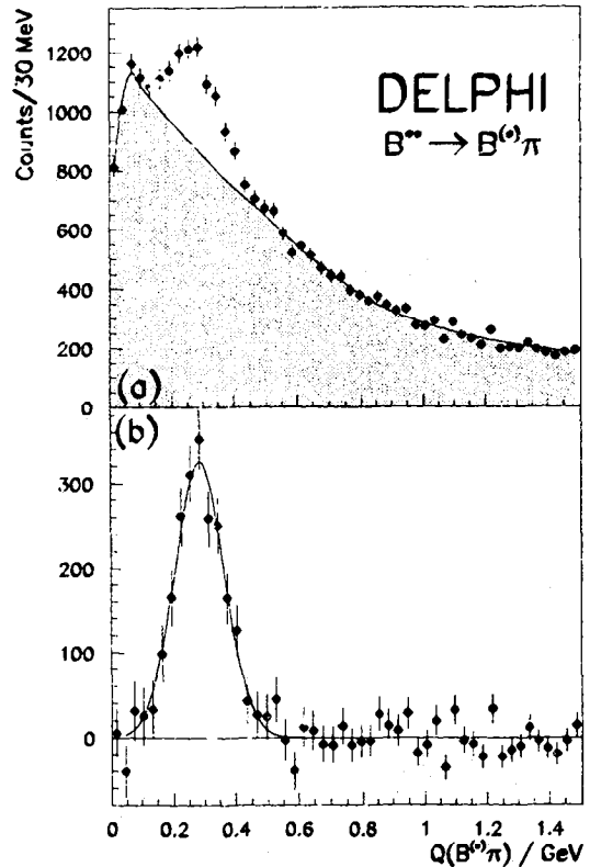
Fig. 1. (a) Distribution of the Q -value of B^{(*)}\pi pairs (data points) along with the Monte Carlo expectation without B^{**} production (shaded area). Q is defined as Q = m(B^{(*)}\pi) - m(B^{(*)}) - m(\pi) . (b) Background subtracted B^{(*)}\pi pair Q -value distribution. The fit is a simple Gaussian.
