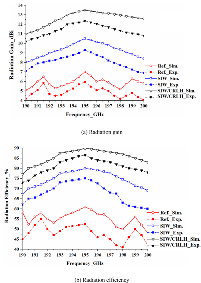
Figure 15. Simulated and experimental results of the radiation gain and efficiency as a function of frequency of the reference, SIW-loaded, and SIW-loaded MTM (CRLH) antenna arrays.
