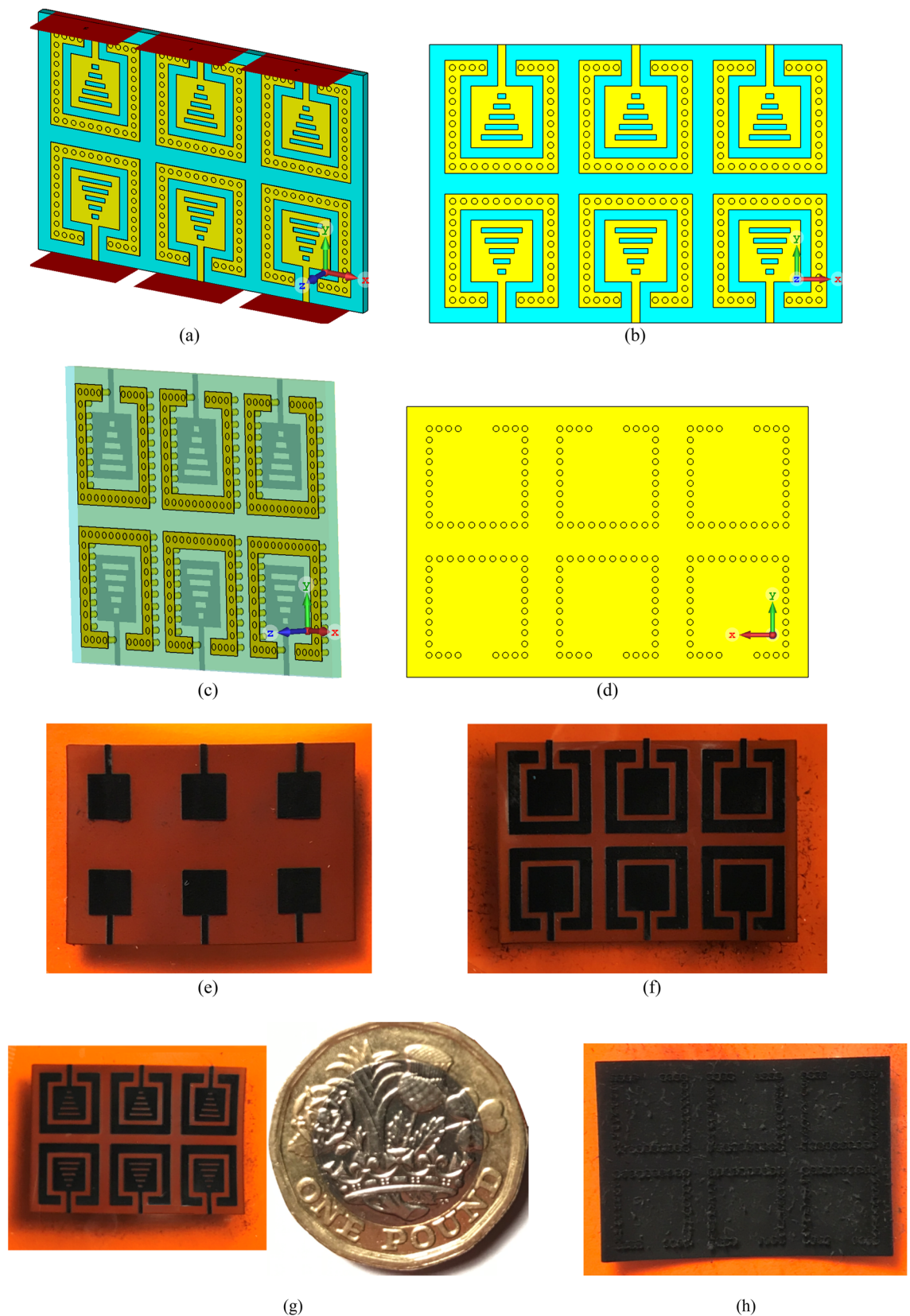
Figure 12. Proposed Graphene coated 2 \times 3 antenna array based on SIW-loaded MTM patches, (a) isometric view, (b) front view, (c) SIW isolators framing the radiation patches, (d) back view (ground-plane), and (e–h) the fabricated antenna array prototype of the reference, SIW-loaded, SIW-loaded MTM antenna, and the ground-plane, respectively.
