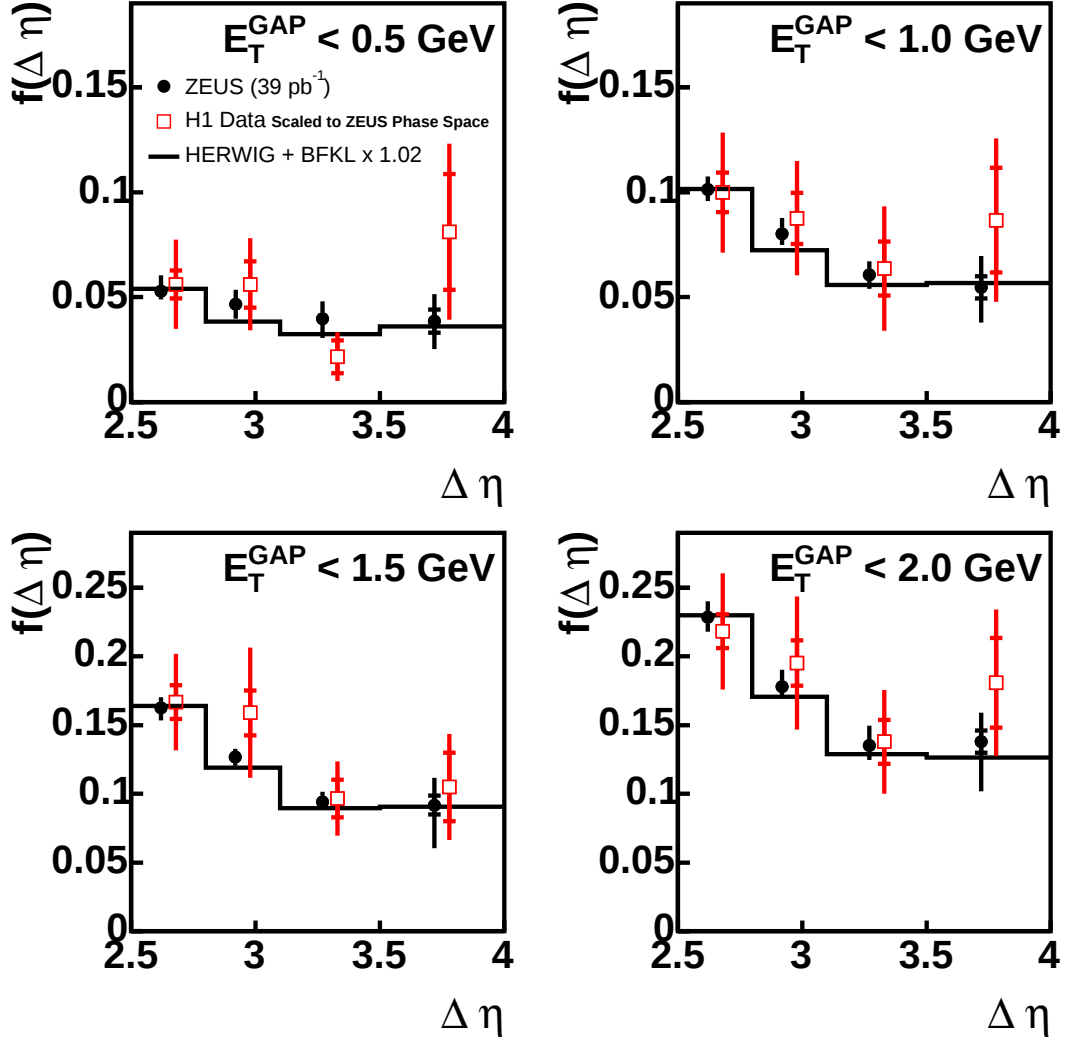
Figure 4: The gap fraction, f , as a function of \Delta\eta for different requirements on E_T^{\text{GAP}} . The black circles represent the ZEUS data, with the inner error bars representing the statistical errors and the outer error bars representing the statistical and systematic uncertainties added in quadrature. The solid black line shows the prediction of HERWIG plus BFKL Pomeron exchange. The open squares represent the H1 data [5] scaled for comparison to the ZEUS phase space as described in the text.
