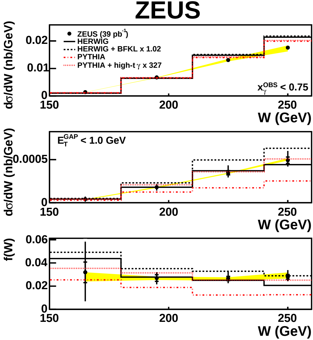
Figure 12: The top plot is the inclusive dijet cross section for x_\gamma^{\text{OBS}} < 0.75 differential in W , the middle plot is the corresponding gap cross section differential in W requiring that E_T^{\text{GAP}} < 1 GeV, and the bottom plot is the gap fraction, f , as a function of W . Other details as in Fig. 1.
