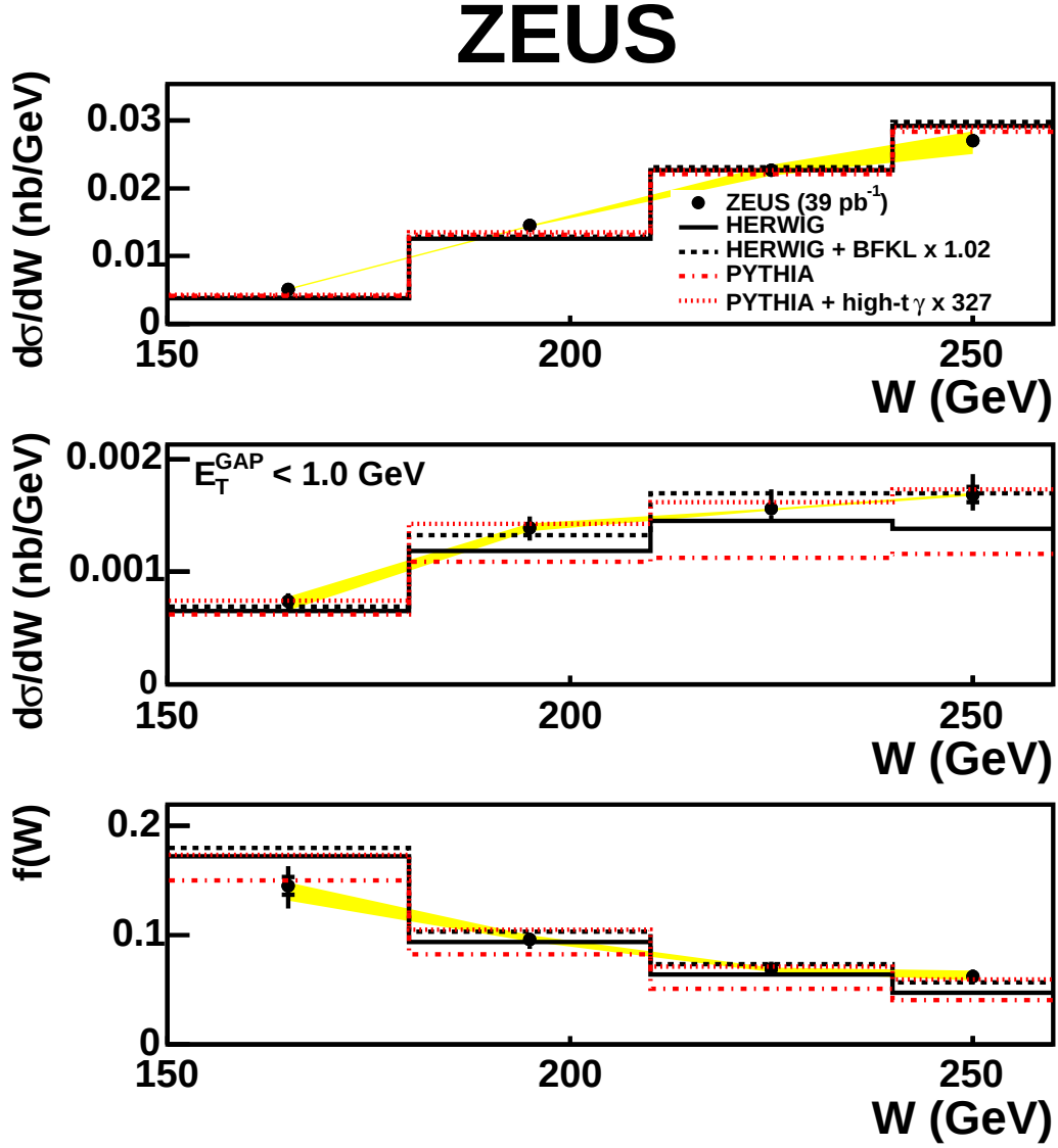
Figure 8: The top plot is the inclusive dijet cross section differential in W , the middle plot is the gap cross section differential as a function of W requiring that E_T^{\text{GAP}} < 1 GeV, and the bottom plot is the gap fraction, f , as a function of W . Other details as in Fig. 1.
