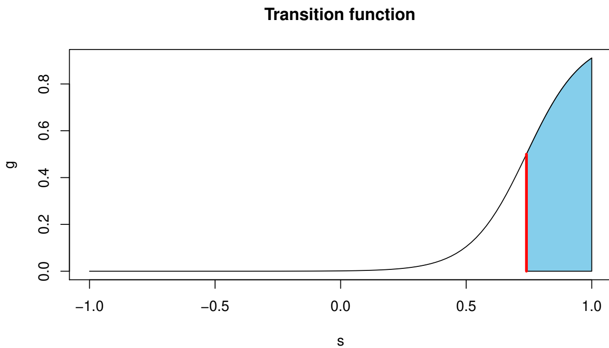
Figure 4: Estimated transition function. The vertical red line indicates the line s = \hat{\tau} = 0.746 , for which g(s_t) = 1/2 . Values above this line, i.e. the shaded area, are interpreted as the bubble regime.
