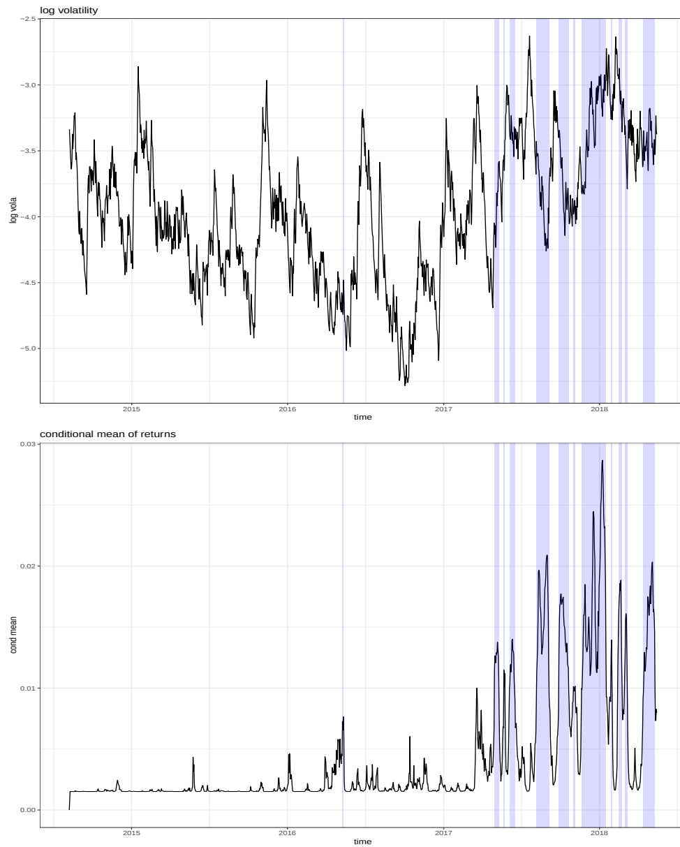
Figure 3: Estimated log volatility (upper panel) and conditional mean (lower panel). The shaded areas correspond to the estimated bubble periods.
