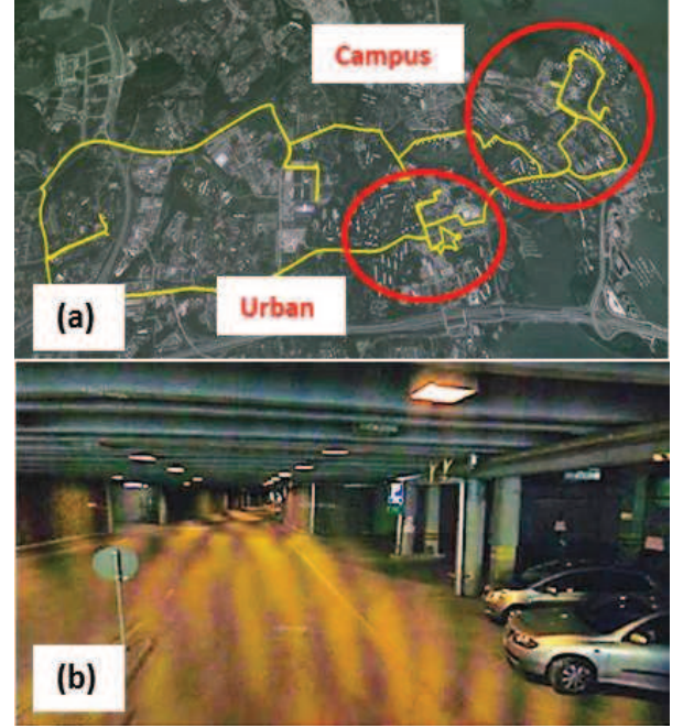
Fig. 2. (a) Top view of measurement routes. The urban and campus areas are marked, and the remaining routes are in suburban area. (b) Underground (tunnel-like) parking scenario, which is located in the urban area.
