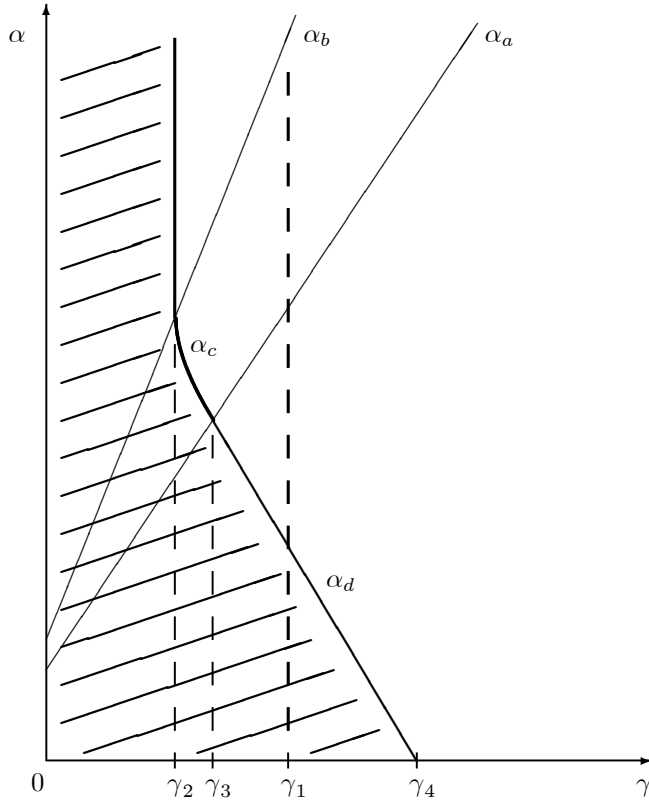
Figure 4 : The equilibrium (0,0)
