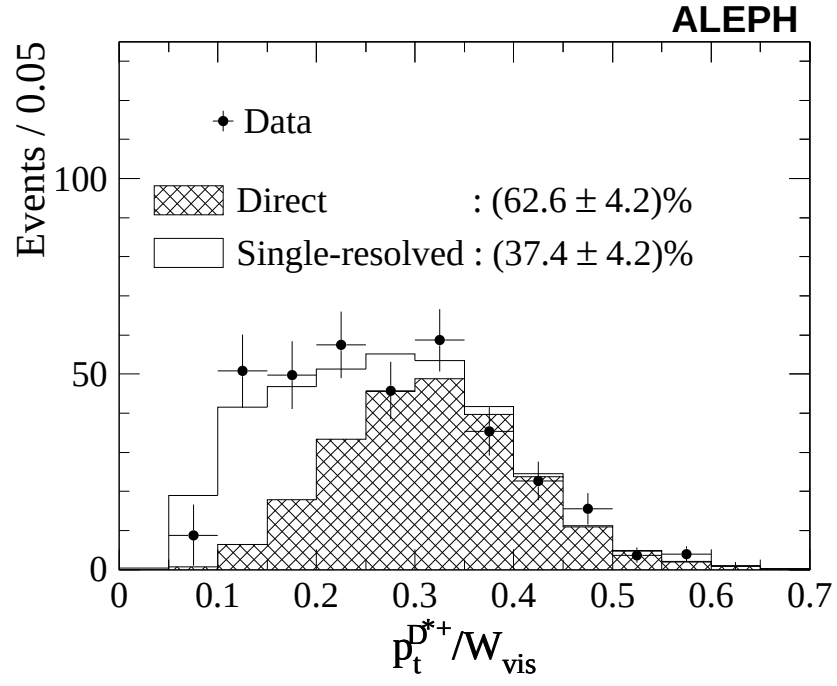
Figure 4: p_t^{D^{*+}}/W_{\text{vis}} distribution for reconstructed D^{*+} events. The points with error bars show data. The relative contributions from direct (shaded histogram) and single-resolved (open histogram) processes are extracted by means of a fit.
