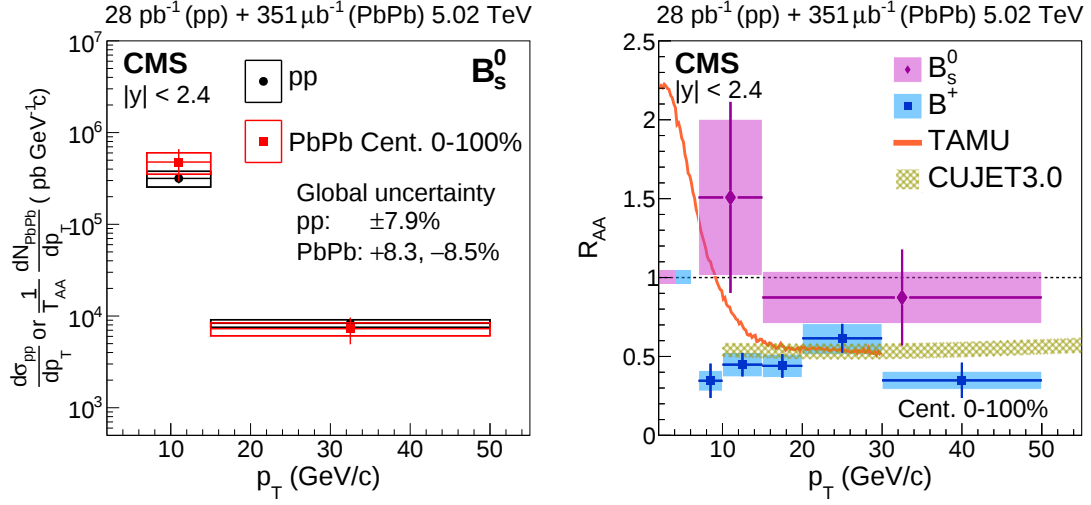
Figure 4: (left) The p_T -differential production cross section of B_s^0 mesons in pp collisions and the p_T -differential corrected yield of B_s^0 mesons scaled by T_{AA} in PbPb collisions at \sqrt{s_{NN}} = 5.02 TeV in two p_T intervals from 7 to 50 GeV/c. The vertical bars (boxes) correspond to statistical (systematic) uncertainties. The systematic uncertainty boxes here include both the correlated and uncorrelated contributions added in quadrature. The global systematic uncertainty comprises the uncertainties in T_{AA} , N_{MB} , and \mathcal{B} . (right) The nuclear modification factor R_{AA} of B_s^0 measured in PbPb collisions at \sqrt{s_{NN}} = 5.02 TeV from 7 to 50 GeV/c. The vertical bars (boxes) correspond to statistical (systematic) uncertainties. The B^+ R_{AA} measurement [29] is also shown for comparison. The global systematic uncertainty, represented by colored boxes at R_{AA} = 1 , comprises the uncertainties in the integrated luminosity measurement and T_{AA} value. Two theoretical calculations are also shown for comparison: TAMU [19, 49] and CUJET3.0 [46–48]. The line width of the theoretical calculation from Refs. [19, 49] represents the size of its statistical uncertainty.
