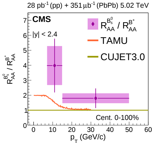
Figure 5: Nuclear modification factor R_{AA} ratio between B_s^0 and B^+ measured in PbPb collisions at \sqrt{s_{NN}} = 5.02 TeV from 7 to 50 GeV/c. Two theoretical calculations are also shown for comparison: TAMU [19, 49], and CUJET3.0 [46–48].
