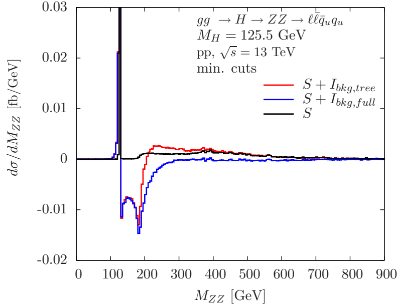
Figure 13. Invariant ZZ mass distributions for the signal process gg \rightarrow H \rightarrow ZZ \rightarrow \ell\bar{\ell}q_uq_u and including its interference with the background in pp collisions at \sqrt{s} = 13 \text{ TeV} . Minimal cuts are applied (see main text). Other details as in figure 12.
