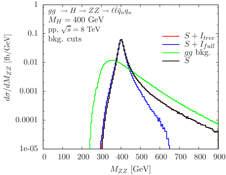
Figure 20. Invariant ZZ mass distributions for the signal process gg \rightarrow H \rightarrow ZZ \rightarrow \ell\bar{\ell}q_uq_u and including its interference with the background in pp collisions at \sqrt{s} = 8 \text{ TeV} with background suppression cuts for a 400 GeV SM Higgs boson (see main text). The gg background is also displayed. Other details as in figure 12.
