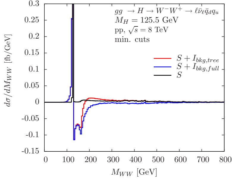
Figure 5. Invariant WW mass distributions for the signal process gg \rightarrow H \rightarrow W^- W^+ \rightarrow \ell \bar{\nu}_\ell q_u \bar{q}_d ( S ) and including its interference with the tree-level ( S + I_{bkg,tree} ) and in addition quark-loop ( S + I_{bkg,full} ) gg background contributions in pp collisions at \sqrt{s} = 8 \text{ TeV} for a 125.5 GeV SM Higgs boson. Minimal cuts are applied (see main text). Other details as in table 1.
