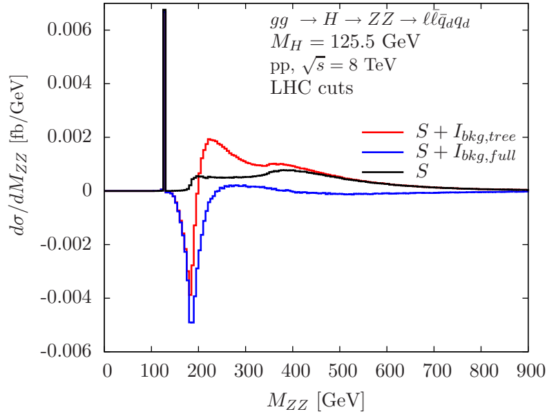
Figure 18. Invariant ZZ mass distributions for the signal process gg \rightarrow H \rightarrow ZZ \rightarrow \ell\bar{\ell}q_d\bar{q}_d and including its interference with the background in pp collisions at \sqrt{s} = 8 TeV. LHC cuts are applied (see main text). Other details as in figure 12.
