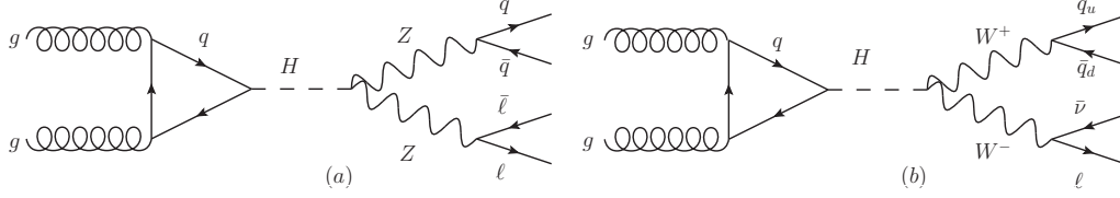
Figure 1. Representative Feynman diagrams for the signal processes considered: (a) gg \rightarrow H \rightarrow ZZ \rightarrow \ell\bar{\ell}q\bar{q} ( q can be an up- or down-type quark, q_{u,d} ) and (b) gg \rightarrow H \rightarrow WW \rightarrow \ell\bar{\nu}_\ell\bar{q}_d q_u (the charge-conjugated process is also considered).
