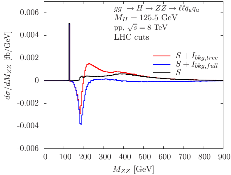
Figure 16. Invariant ZZ mass distributions for the signal process gg \rightarrow H \rightarrow ZZ \rightarrow \ell\bar{\ell}q_u\bar{q}_u and including its interference with the background in pp collisions at \sqrt{s} = 8 \text{ TeV} . LHC cuts are applied (see main text). Other details as in figure 12.
