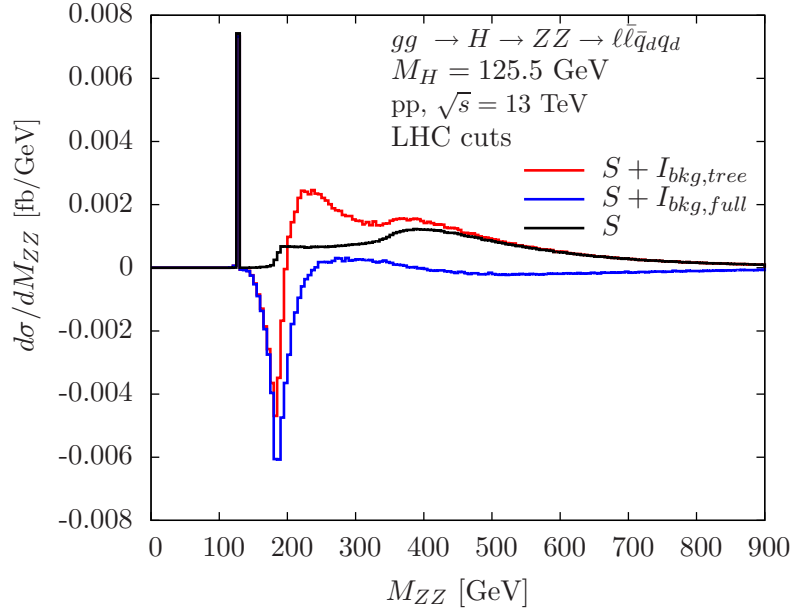
Figure 19. Invariant ZZ mass distributions for the signal process gg \rightarrow H \rightarrow ZZ \rightarrow \ell\bar{\ell}q_dq_d and including its interference with the background in pp collisions at \sqrt{s} = 13 \text{ TeV} . LHC cuts are applied (see main text). Other details as in figure 12.
