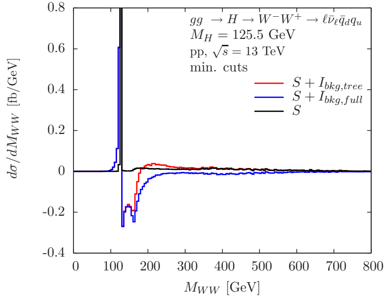
Figure 6. Invariant WW mass distributions for the signal process gg \rightarrow H \rightarrow W^- W^+ \rightarrow \ell \bar{\nu}_\ell q_u \bar{q}_d and including its interference with the background in pp collisions at \sqrt{s} = 13 \text{ TeV} . Minimal cuts are applied (see main text). Other details as in figure 5.
