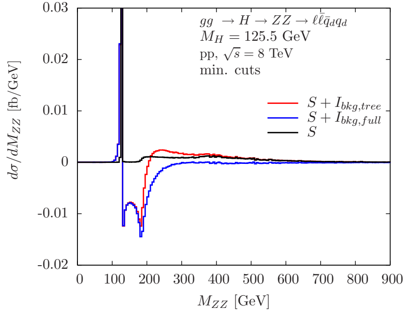
Figure 14. Invariant ZZ mass distributions for the signal process gg \rightarrow H \rightarrow ZZ \rightarrow \ell\bar{\ell}q_dq_d and including its interference with the background in pp collisions at \sqrt{s} = 8 \text{ TeV} . Minimal cuts are applied (see main text). Other details as in figure 12.
