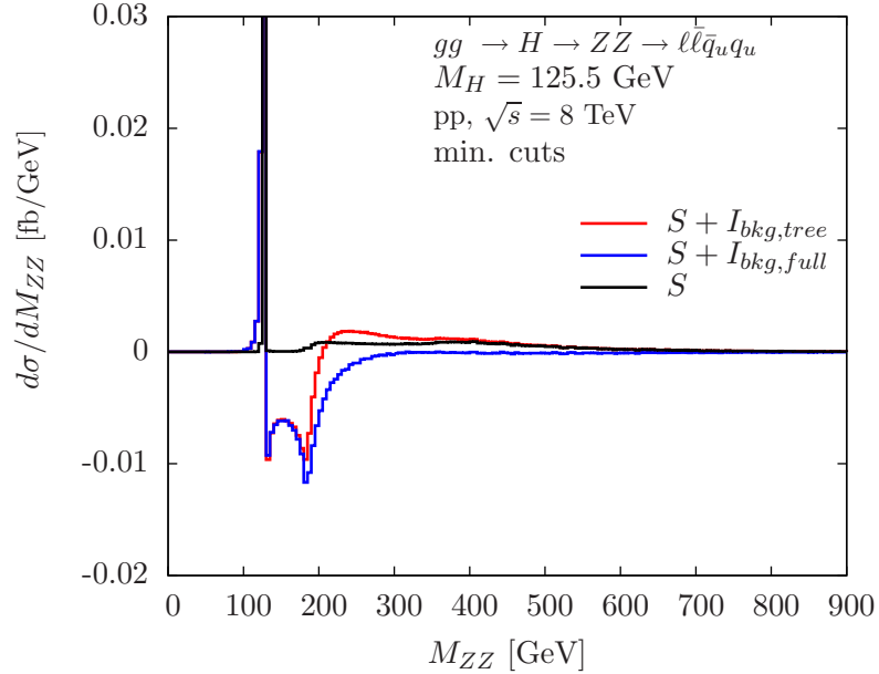
Figure 12. Invariant ZZ mass distributions for the signal process gg \rightarrow H \rightarrow ZZ \rightarrow \ell\bar{\ell}q_u \bar{q}_u and including its interference with the background in pp collisions at \sqrt{s} = 8 TeV. Minimal cuts are applied (see main text). \gamma^* background contributions are included. Other details as in figure 5.
