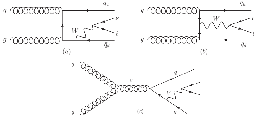
Figure 2. Representative tree-level background diagrams of \mathcal{O}(g_s^2 e^2) that interfere with the signal diagrams in figure 1.
