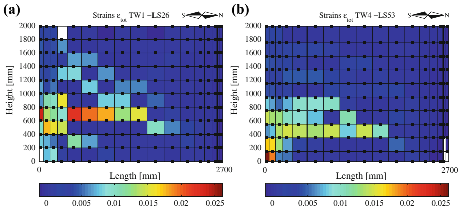
Fig. 19 Distribution of 'local' axial strain (positive values refer to tensile strains) throughout the test units at the first cycle at 0.75 % in-plane and 0 % out-of-plane drift, when the web edge is in tension: a wall TW1 (LS26); b wall TW4 (LS53)
