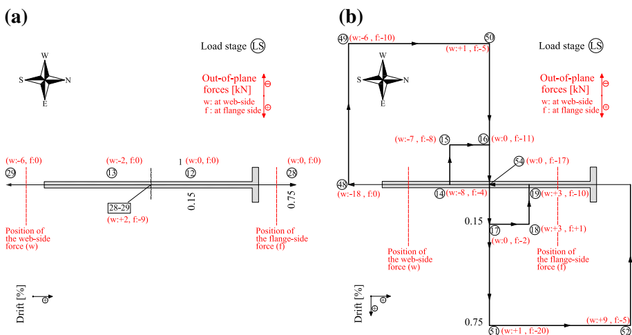
Fig. 15 Identification of the out-of-plane forces at the top beam level, at the web (w) and flange (f) side, in two illustrative cycles (0.15 % and 0.75 % drift): a internal forces in the steel tubes used in TW1 test; b forces in the out-of-plane actuators in TW4 test
