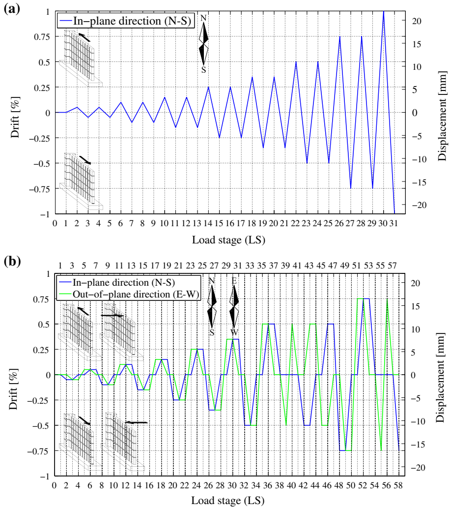
Fig. 5 Drift protocols of the two quasi-static cyclic tests, including load stages (LS): a wall TW1; b wall TW4
