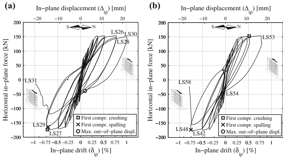
Fig. 9 In-plane force–displacement response: a wall TW1; b wall TW4
