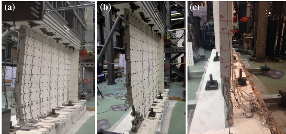
Fig. 7 a Deformed shape of wall TW1 at loading LS30 → LS31, around 0 % in-plane drift; b wall TW1 at the end of the test, after failure; c wall TW4 at the end of the test, after failure
