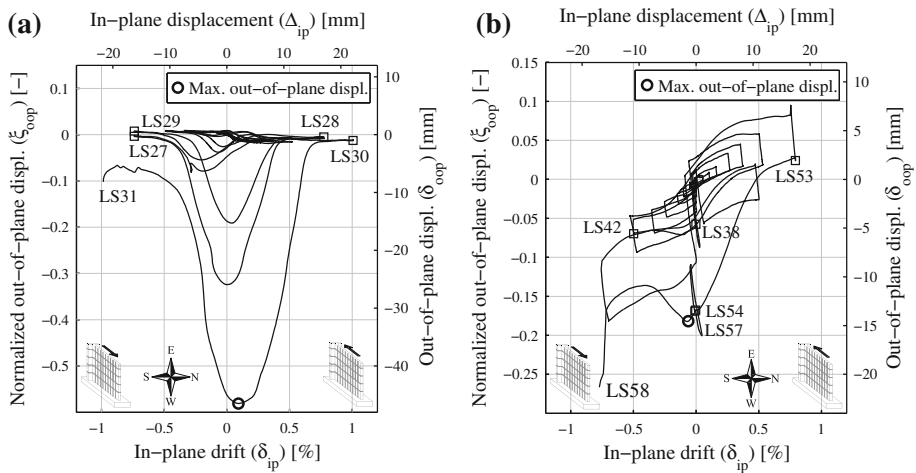
Fig. 10 Imposed in-plane drift versus normalized web edge out-of-plane displacement at the height where maximum out-of-plane displacement was measured, i.e. at marker no. 7 in Fig. 4b: a wall TW1; b wall TW4
