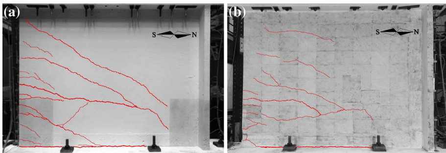
Fig. 18 Crack pattern on the West side of the test units, when they were loaded at 0.75 % in-plane and 0 % out-of-plane drift: a wall TW1 (LS26); b wall TW4 (LS53)
