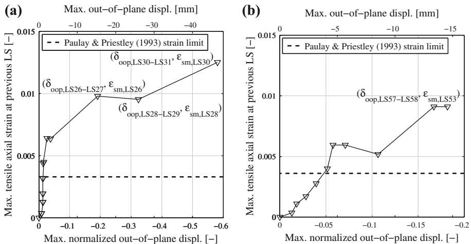
Fig. 16 Maximum out-of-plane displacement attained between each two consecutive LS versus axial tensile strain attained at previous LS with web edge in tension: a wall TW1; b wall TW4 (only LS at 0 % out-of-plane drift are presented in this figure)
