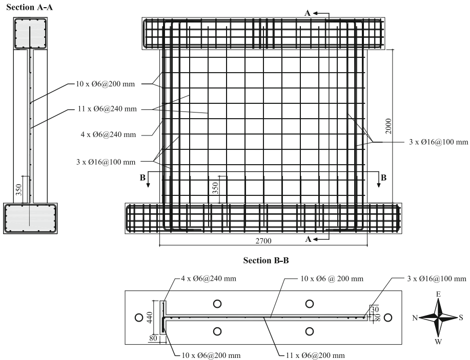
Fig. 3 Geometrical characterization and detailing of test units TW1 and TW4 (all dimensions in mm)
