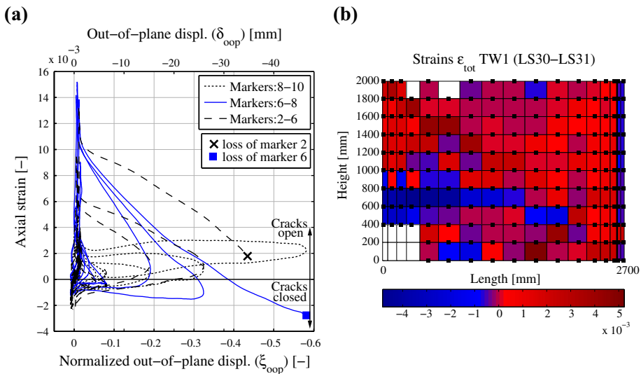
Fig. 17 TW1: a out-of-plane displacement versus ‘local’ axial strain as computed between the indicated pairs of LEDs; b Distribution of axial strain throughout the wall when the maximum out-of-plane displacement was attained (during loading LS30 → LS31, at \xi_{oop} = 0.518 )
