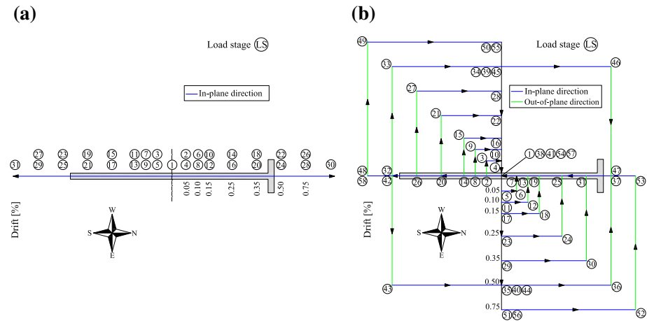
Fig. 6 In-plane representation of the two loading protocols, including load stages (LS): a wall TW1; b wall TW4
