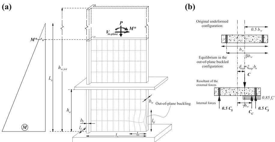
Fig. 2 a Wall geometrical characterization; b illustration of one possible equilibrium state between external and internal forces at mid-height of buckling region, adapted from Paulay and Priestley (1993)
