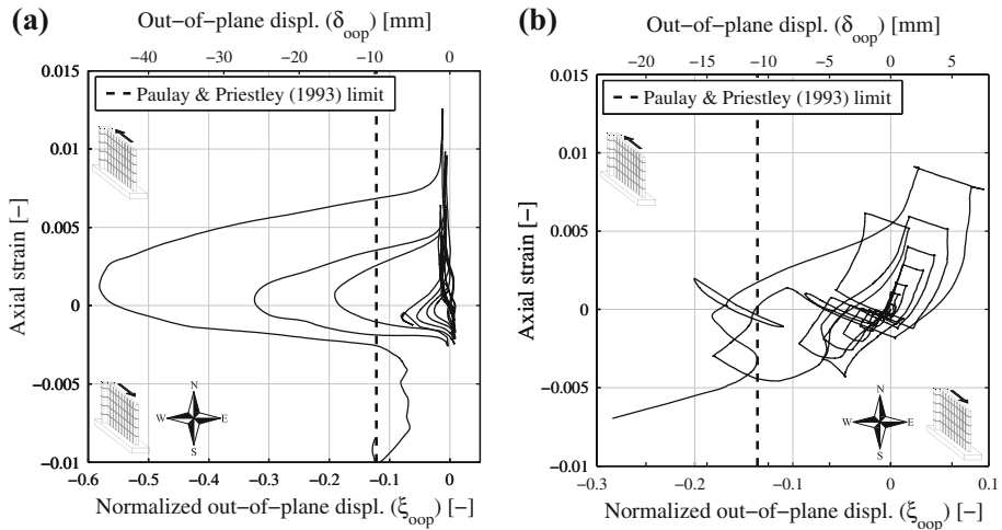
Fig. 11 Normalized out-of-plane displacement versus axial strain (computed between LEDs no. 222 and no. 239, see Fig. 4b): a wall TW1; b wall TW4
