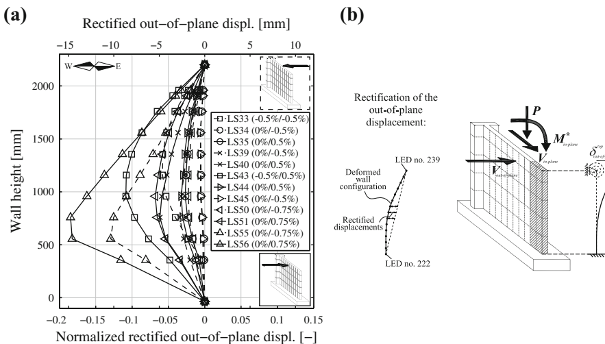
Fig. 14 a Rectified normalized web edge out-of-plane displacement profile along the wall height at specific load stages for wall TW4, when out-of-plane drift was different from 0 % (in-plane/out-of-plane drifts are indicated in parentheses). b Rectification of the out-of-plane displacements and equivalent beam model for wall web edge when an out-of-plane displacement is imposed at the top of the wall
