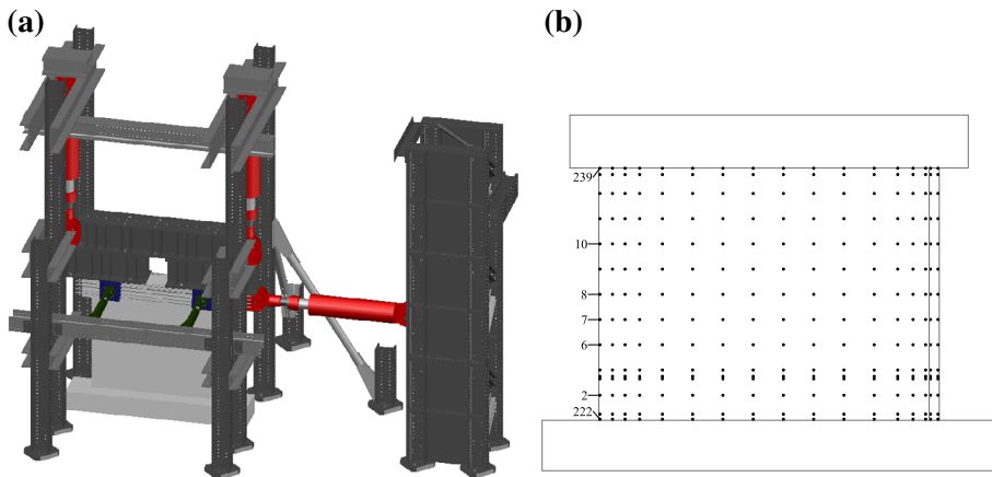
Fig. 4 a 3D representation of the test setup; b LED grid used for the optical measurement system (with identification of LEDs no. 6, no. 7, no. 8, no. 10 no. 222, and no. 239 at the wall web edge)
