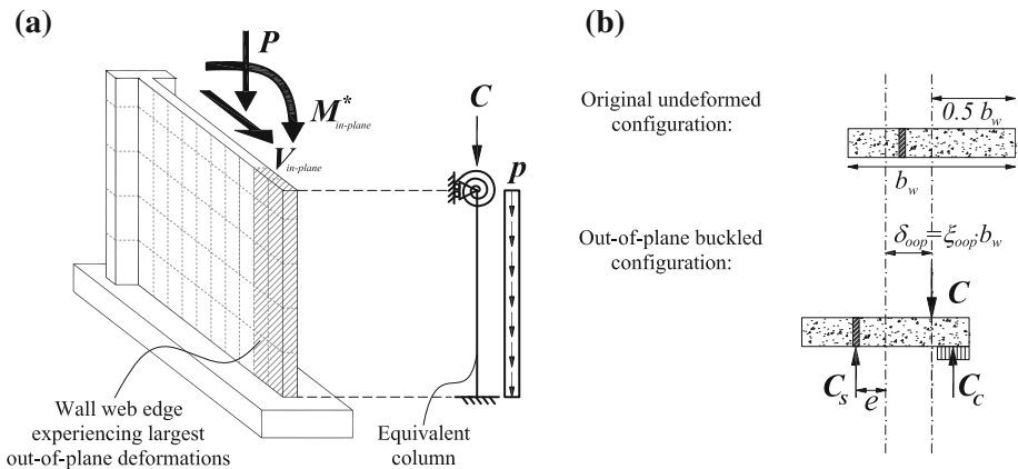
Fig. 8 a Equivalent beam model for wall web edge with applied loads and boundary conditions. b Illustration of one possible equilibrium state at midheight of buckling region for a wall with a single layer of longitudinal reinforcement
