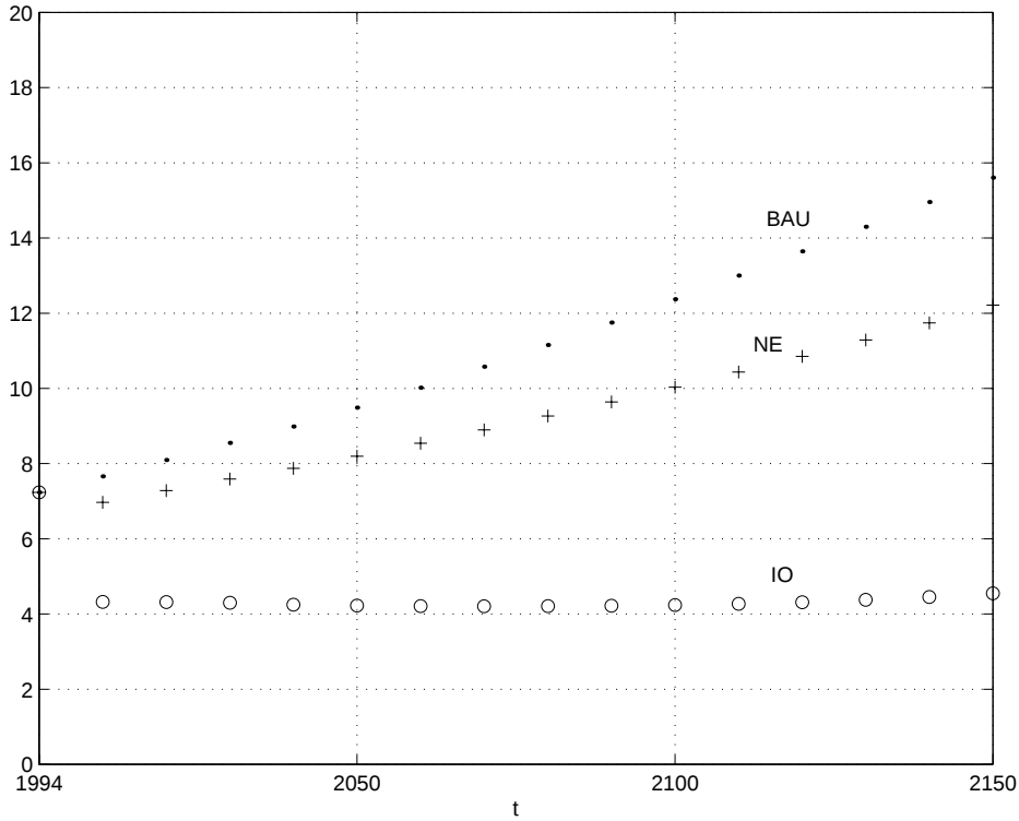
Figure 1 : average annual world carbon emissions (in GtC/year)
