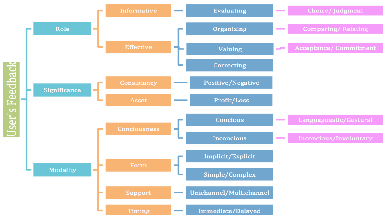
Figure3. A user's Feedback Ontology
