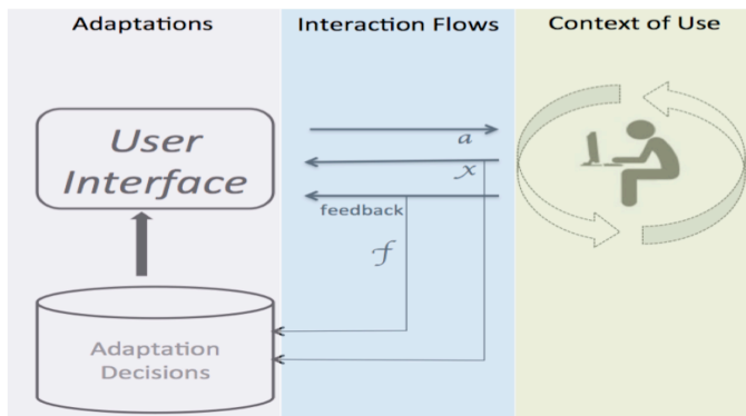
Figure2. Model of intelligent adaptation based on user's Feedback
