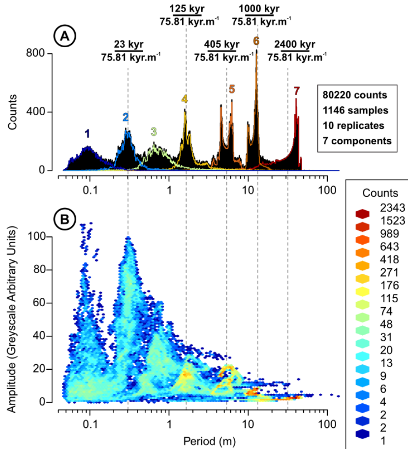
195 Figure SF8: (A) Period distribution and (B) spectral population of the components of CIP1 decomposition (ensemble of 10 replicate decompositions with identical parameters but with different white noise realisations; see also Fig. SF4). The dotted lines stand for the expected periods of climatic precession (ca. 23 kyr), and of climatic precession modulators: short-eccentricity (ca. 125 kyr), long eccentricity (405 kyr), the g_1 - g_5 cycle (ca. 1000 kyr) and the g_4 - g_3 cycle (ca. 2400 kyr) (e.g. Olsen and Kent 1999; Hinnov 2000; Laskar et al. 2011). [NOTE TO REVIEWERS: colour online only; 1.5 column fitting image]
