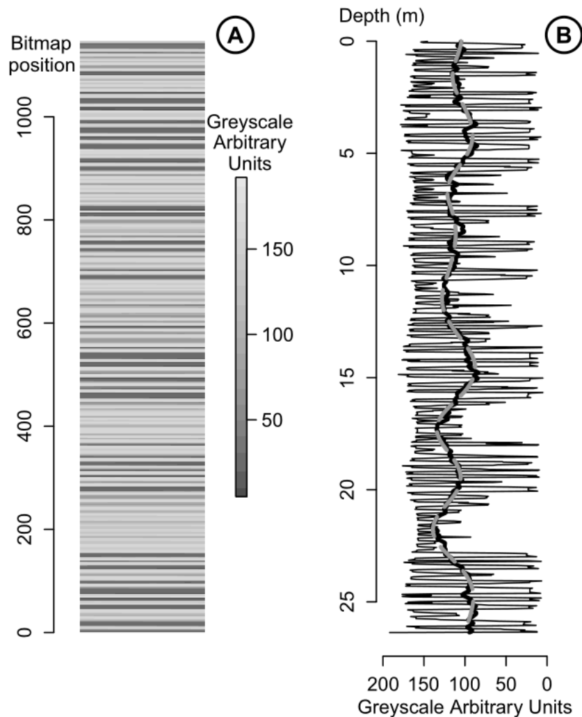
85 Figure SF3: (A) grey-scale version of the CIP1 original signal (image of a supposed core) and (B) its conversion into a proxy record, to which is added a running average of 101 points (bold black line) and an addition of some of the last components obtained via EEMD by "extricate" (bold grey dashed line). These two lines illustrate that the dissymmetry of amplitude modulation translates into raw cycles being poured into the signal by partial rectification (see also section 5.3.1 in Weedon 2003). [NOTE TO REVIEWERS: 1.5 column fitting image]
