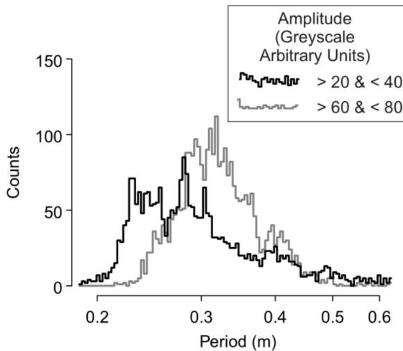
205 Figure SF9: (A) Period distribution of comp. 2 (ensemble of 10 replicate decompositions with identical parameters but with different white noise realisations): the distribution is divided between "low amplitude" (between 20 and 40 greyscale arbitrary units, shown has the black line) and "high amplitude" (between 60 and 80 greyscale arbitrary units; shown has the grey line). The period distribution shifts towards higher values in the "high amplitude" curve, which indicates that sedimentation rate is indeed higher when the amplitude is higher. [NOTE TO REVIEWERS: 1 column fitting image]
