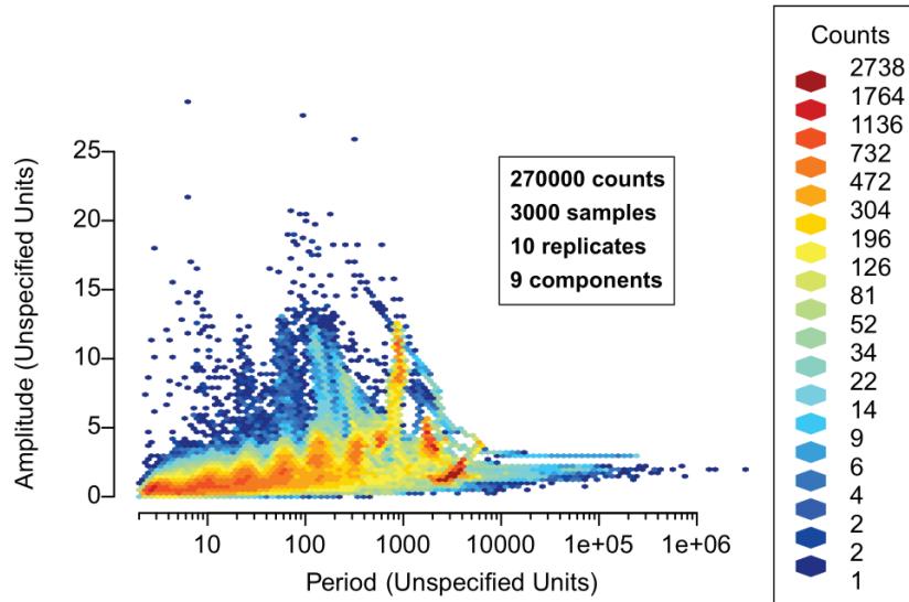
Figure SF1: Spectral population plot of a 3000 point red noise signal. [NOTE TO REVIEWERS: colour online only; 1.5 column fitting image]
