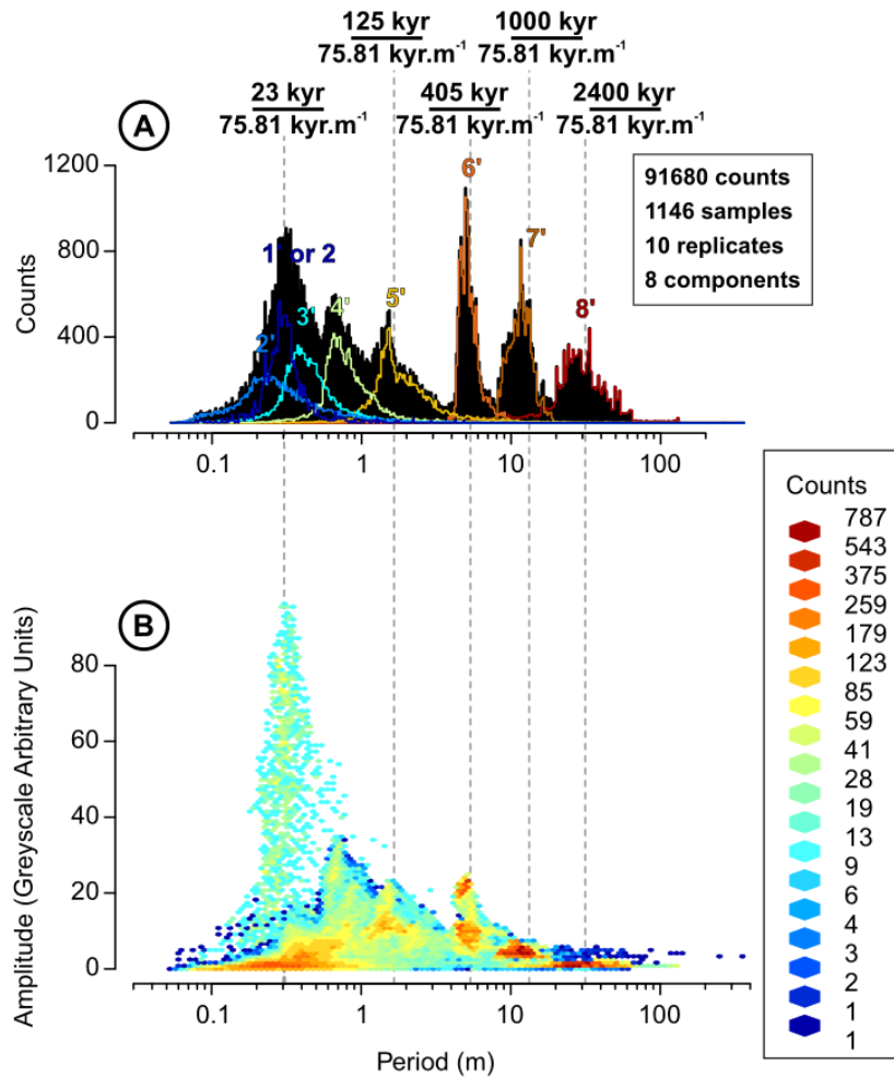
245 Figure SF11: (A) Period distribution and (B) spectral population of the components of the decomposition (ensemble of 10 decompositions with identical parameters but with different white noise realisations) of the amplitude demodulation of one realisation of comp. 2 of the CIP1 signal decompositions (see Fig. 19).
