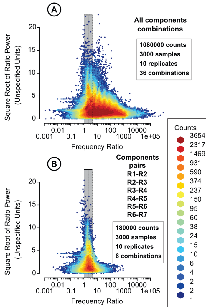
60 Figure SF2: (A) Ratio population for all pairs of components, of the same 3000 points red noise signal used for fig. SF1 (ensemble of 10 decompositions with identical parameters but with different white noise realisations). (B) Ratio population plot of the red noise signal for only the successive components. The grey rectangle delimits frequency ratios between 1 and 4, and is centred on a ratio of 2. [NOTE TO REVIEWERS: colour online only; 1.5 column fitting image]
