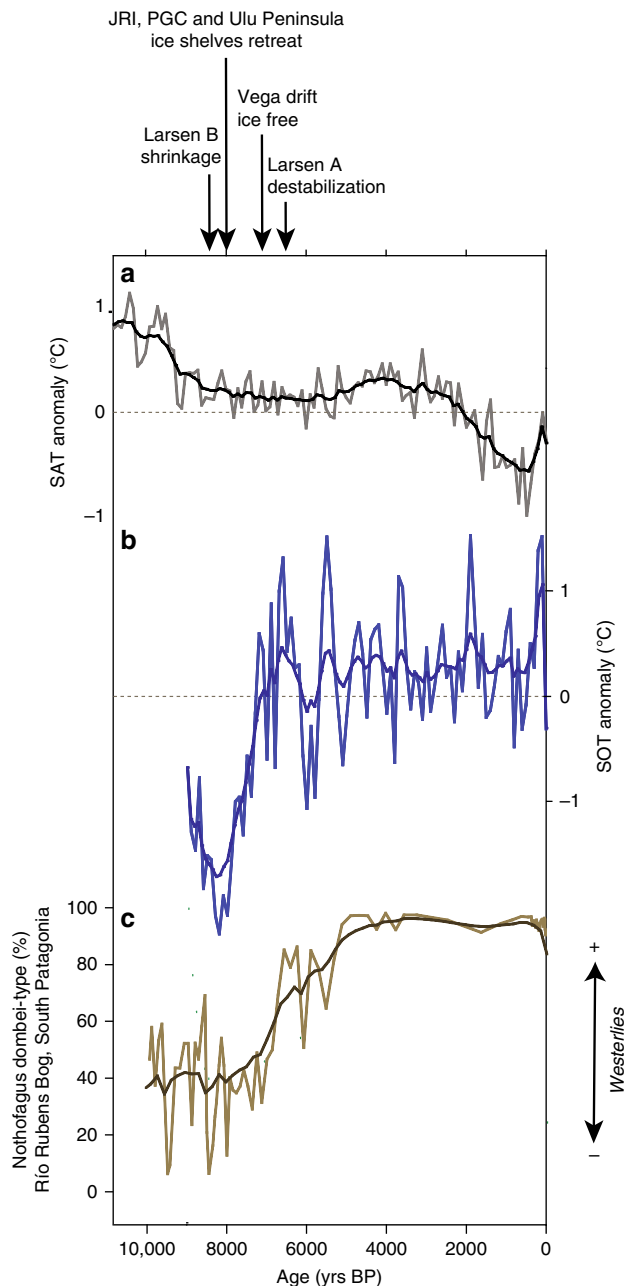
Fig. 3 Holocene SAT, SOT, and SWW records. a The 100-year average SAT anomaly at the JRI core site (gray) 27 , b the 100-year average TEX 86 L -derived SOT anomalies reconstructed at the JPC-38 (blue) and their respective smoothed records spanning the last 9000 years. c Nothofagus pollen record (%) at the Río Rubens Bog site, Patagonia, east of the Andes, Argentina, reflecting intensity and southward migration of the Westerlies 41–43 . The black arrows represent the major steps of the EAP ice shelf history 29–35
