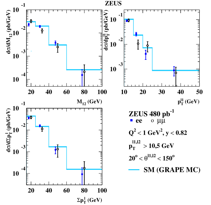
Fig. 5. Differential cross sections as a function of (a) the invariant mass of the lepton pair, M_{12} , (b) the transverse momentum p_T^l of the highest- p_T lepton, and (c) the scalar sum of the transverse momenta of the two highest- p_T leptons, \sum p_T^l . The di-muon cross sections are shown as the open dots, while the full dots are the di-electron measurements, which have been displaced for clarity. The data are compared with the predictions of the GRAPE Monte Carlo. The full error bars are the quadratic sum of the statistical (inner part) and systematic uncertainties.
