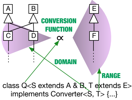
Figure 1: Quantifying over variable types
