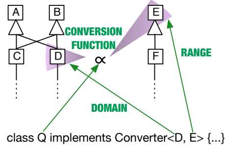
Figure 2: Quantifying over concrete types
