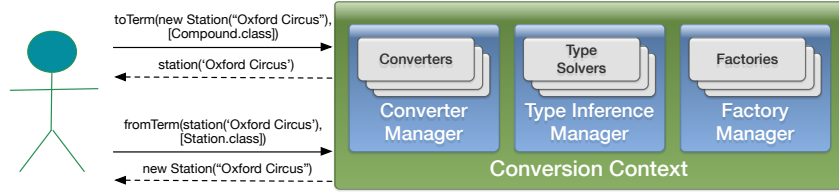
Figure 3: The conversion context
