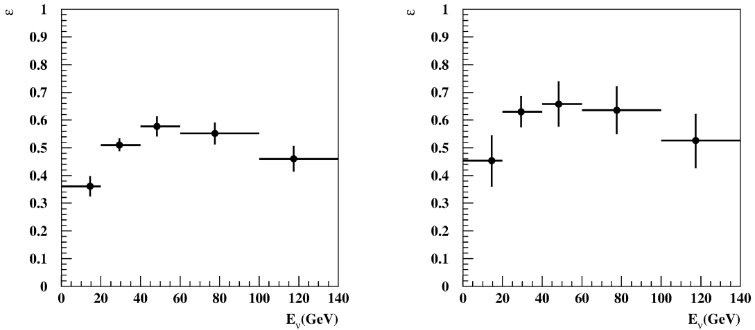
Fig. 2. Detection efficiency as a function of E_\nu for V2 (left) and V4 (right) topologies. The error bars are statistical uncertainties in the simulation.
