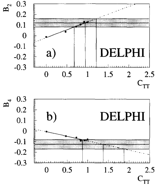
Fig. 4. The full circles show the fitted values of (a) B_2 and (b) B_4 versus the input correlation parameter C_{TT} for events generated with the KORALB Monte Carlo. B_2 was obtained with a fit to data belonging to class II in the hadron-hadron topology, while B_4 with a fit to data belonging to class II in the hadron-lepton topology. Straight line fits are superimposed. The shaded bands correspond to the \pm 1 standard deviation variations of the values measured on the data.
