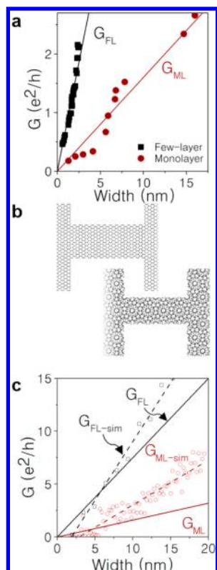
Figure 5. Conductance scaling of GNRs. (a) Measured conductance as a function of width for few-layer (black squares) and monolayer (red circles) GNRs, after subtraction of the best fit contact resistance. The black line is a fit of the form G_{FL}(w) \approx 0.75 (e^2/h)w[\text{nm}] , and the red line is a fit of the form G_{ML}(w) = 0.15 (e^2/h)w[\text{nm}] . (b) Ball and stick models of armchair-edge monolayer (top) and bonded bilayer (bottom) GNR devices used for quantum transport calculations. (c) Conductance as a function of width for simulated and measured GNRs. Black (red) data points are from simulations of the conductance of bonded bilayer (armchair-edge monolayer) GNR with dashed lines as corresponding linear fits. Solid lines represent linear fits to the experimental data, as reproduced from panel (a).
