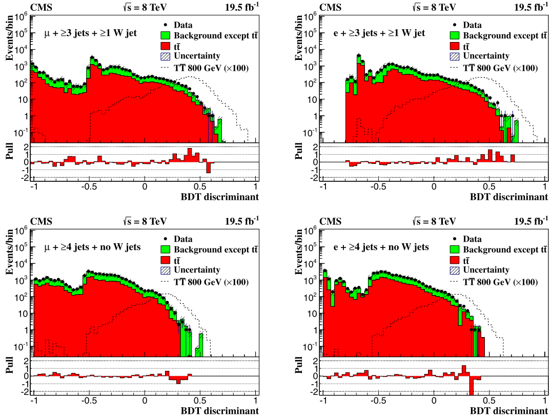
Fig. 2. Observed and expected distributions of the BDT discriminant. The distribution for a T quark with a mass of 800 GeV is also shown. The top panel is for events with at least one W jet, the bottom panel for events without W jets. The left column is for events with a muon and the right column for events with an electron.
