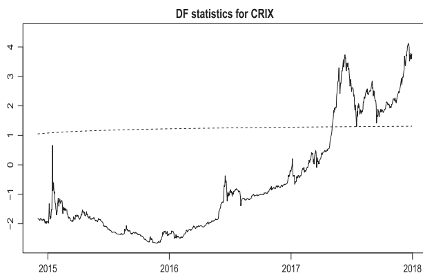
Figure 4 Time series of recursive DF_r statistics for CRIX. The dashed line is the function \log(\log(T_r))/1.5 , r \in [0.1, 1] giving the critical value as a function of the sample size and corresponding roughly to the 1% upper quantile of the DF_1 distribution.
