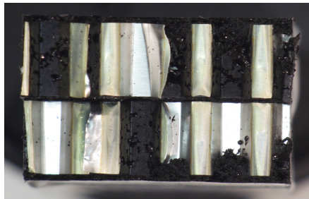
(c) double wall oriented perpendicularly to the direction of the beam.
