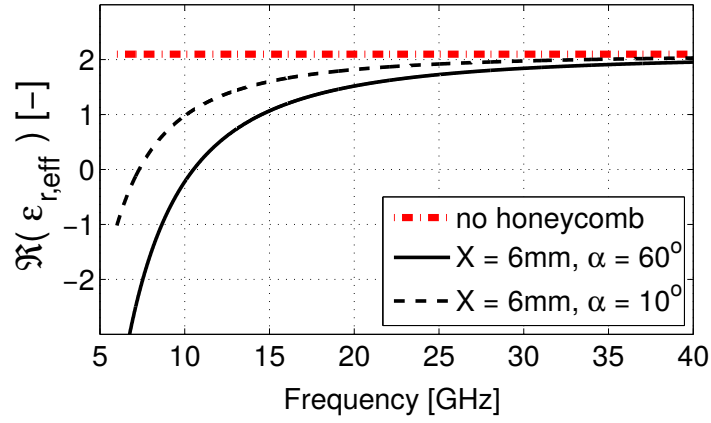
Figure 4.3: Effect of the angle of the honeycomb on \Re(\varepsilon_{r,eff}) calculated with X = 6\text{mm} , \varepsilon_r = 2.1 , \sigma = 1 \text{ S/m} , m = 1 and n = 0 in equation (4.11).
