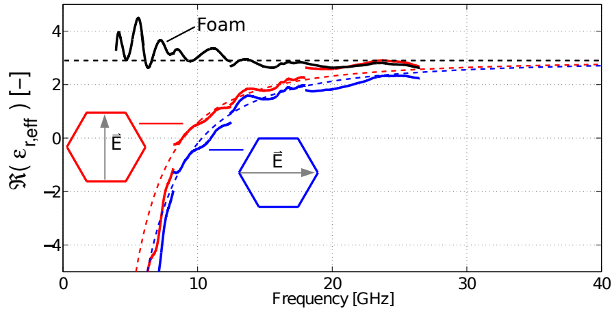
Figure 4.15: Experimental measurement and analytical effective permittivity for 0^\circ and 90^\circ polarisation angle.
