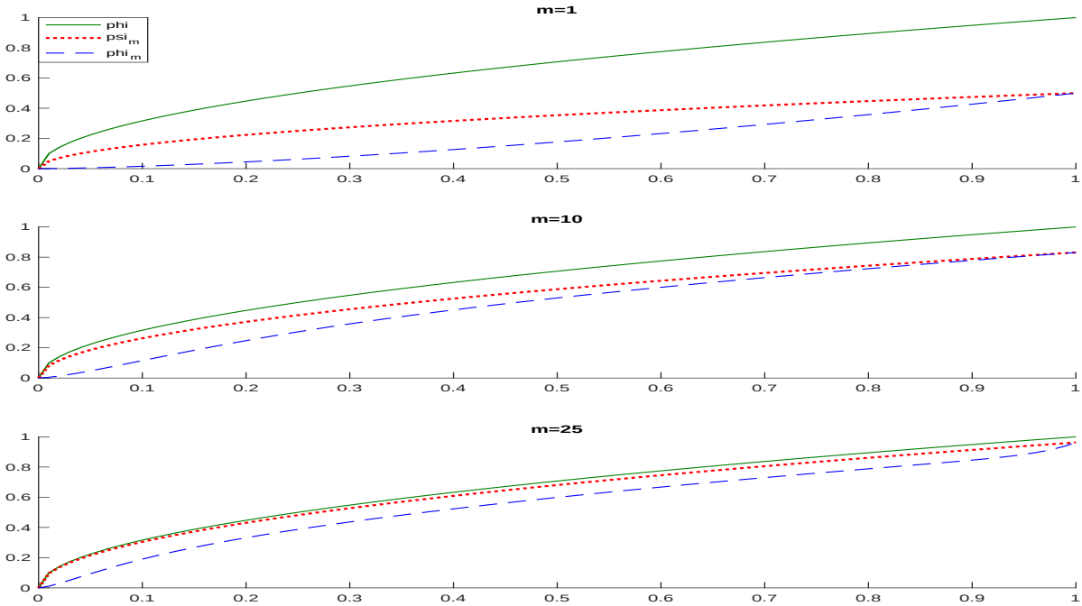
Figure 7: Cobb-Douglas example—Same graphs as before.
