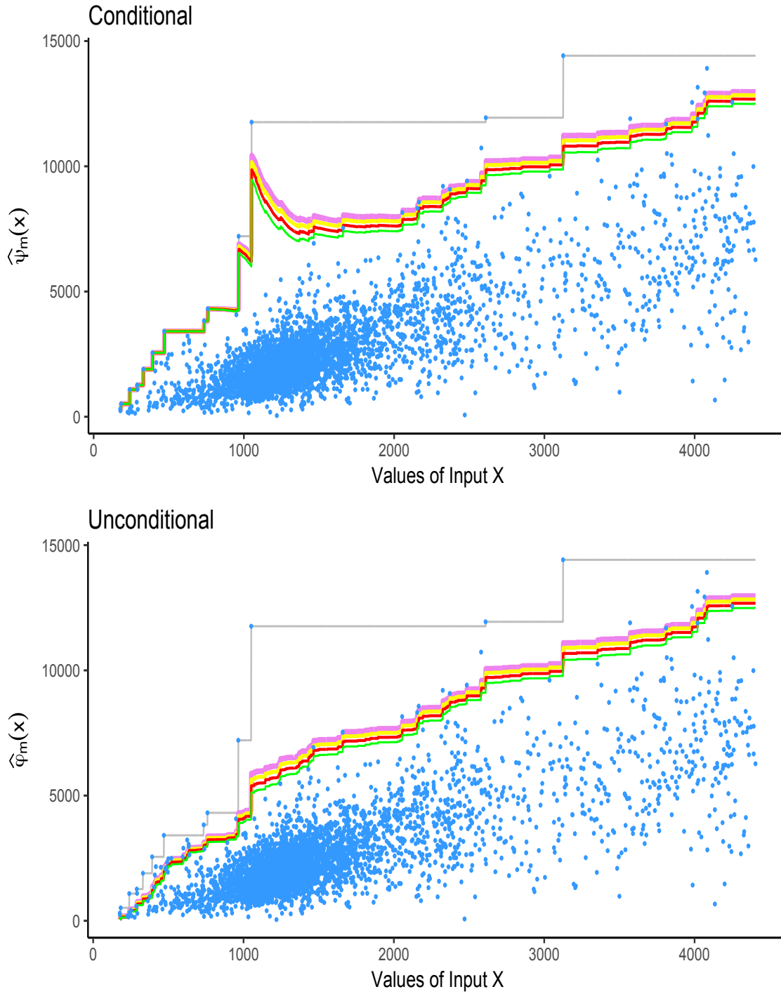
Figure 2: Scatterplot of the n = 4,000 delivery post offices—Estimated expected maximum production frontiers \hat{\psi}_m (top) and \hat{\varphi}_m (bottom), with m = 600, 700, 800, 900 and m = \infty (FDH), respectively, in green, red, yellow, violet and gray curves.
