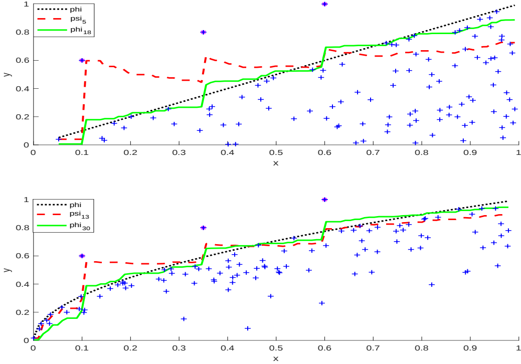
Figure 10: Typical realizations for simulated samples of size n = 100 . Top—Uniform triangle example. Bottom—Cobb-Douglas example. True frontier \varphi in dotted line with its optimal m -frontier estimators \hat{\psi}_m in dashed line and \hat{\varphi}_m in solid line.
