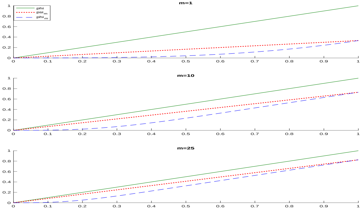
Figure 6: Uniform triangle example—Graphs of \varphi in solid line, \psi_m in dotted line, and \varphi_m in dashed line.
