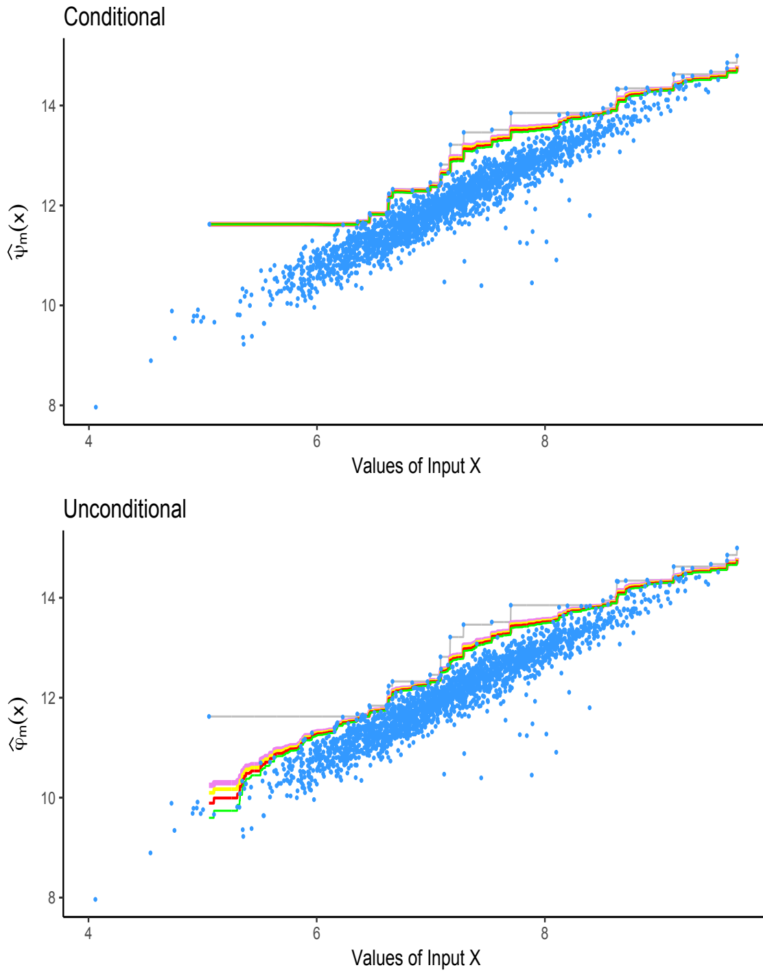
Figure 1: Scatterplot of the n = 2,326 delivery post offices (data in logarithms)—Estimated expected maximum production frontiers \hat{\psi}_m (top) and \hat{\varphi}_m (bottom), with m = 600, 700, 800, 900 and m = \infty (FDH), respectively, in green, red, yellow, violet and gray curves.
