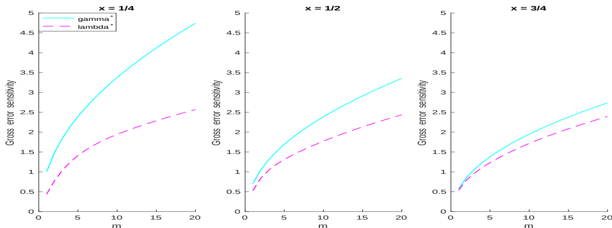
Figure 9: Cobb-Douglas example —Gross-error sensitivities plots as before.
