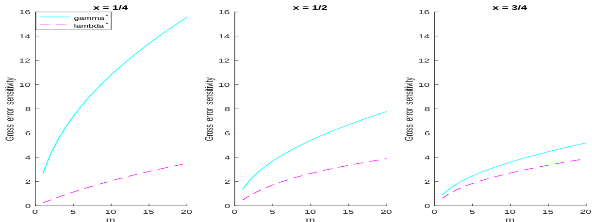
Figure 8: Uniform triangle example —Gross-error sensitivities m \mapsto \gamma^*(T_m^x, F_{(X,Y)}) in solid line and m \mapsto \lambda^*(T_m, F_{Y^x}) in dashed line.
