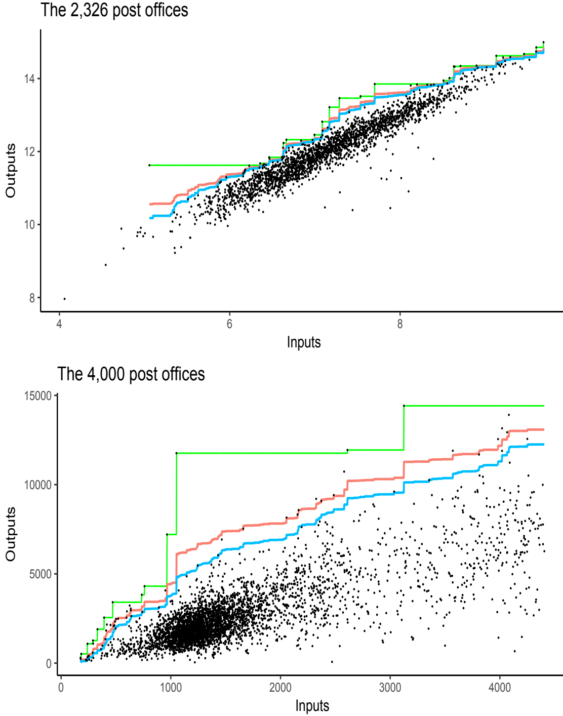
Figure 5: Selected (lower and upper) expected maximum production frontiers \hat{\varphi}_m . Top—dataset of size 2,326 in logarithms, with m = 1250 (upper) in red line, m = 850 (lower) in blue line, and m = \infty (FDH) in green line. Bottom—dataset of size 4,000, with m = 1000 (upper) in red line, m = 500 (lower) in blue line, and m = \infty (FDH) in green line.
