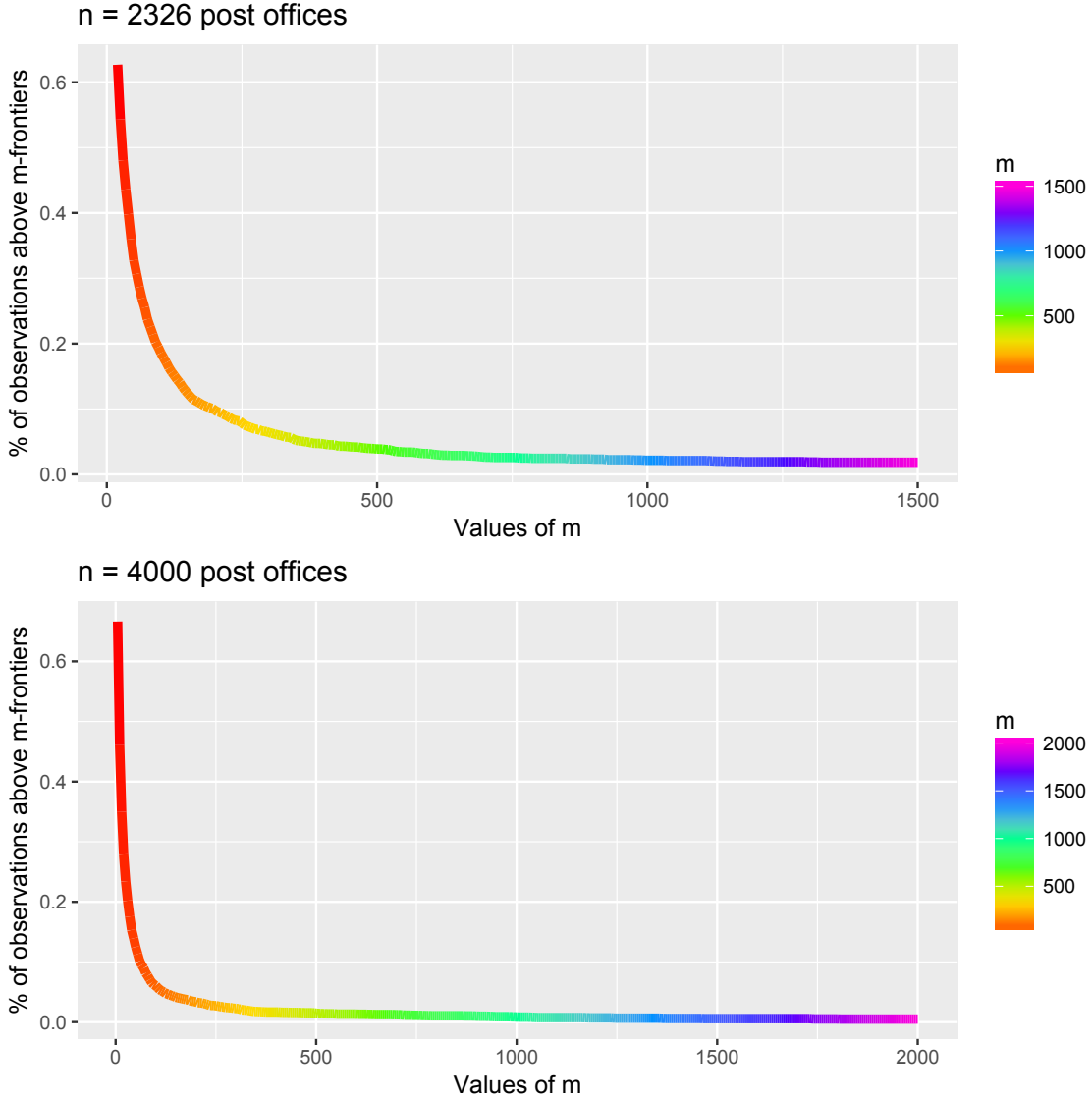
Figure 4: Evolution of the % of sample points outside the partial m -frontiers \hat{\varphi}_m .
