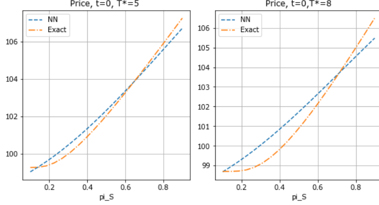
Figure 6: Comparison of exact and PINN prices of a 5 and 8-year GMAB with: S_0 = 100 , \pi_S \in [0, 1] and \pi_D = \pi_M = \frac{1-\pi_S}{2} . (r_0, \mu_0, \lambda_0) of Table 2.
