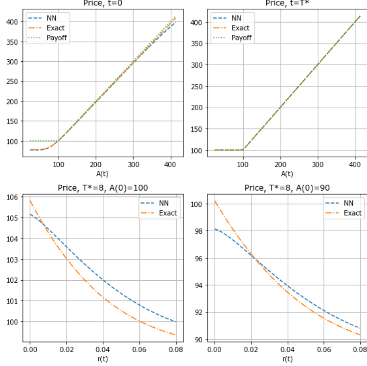
Figure 2: Comparison of exact and PINN prices of a T^* = T = 8 years GMAB with: A_0 = 100 , \pi = (0.50, 0.25, 0.25) , (r_0, \mu_0, \lambda_0) of Table 2. Upper plots: values at issuance and expiry, for A_t \in [23.82, 414.15] . Lower plots: values at issuance with A_0 = 100 and 90 , for r_0 \in [0.00, 0.08] .
