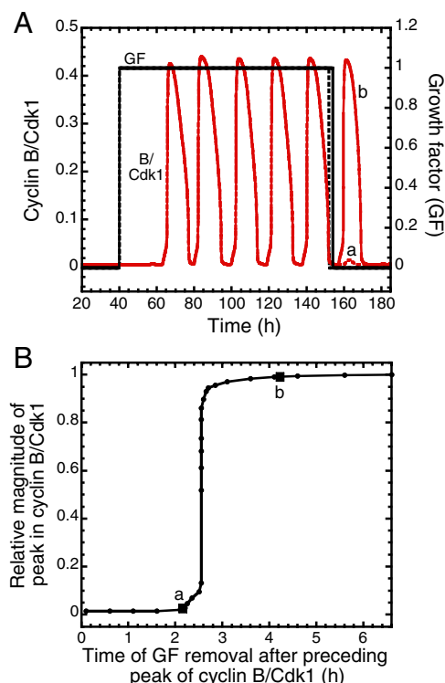
Fig. 3. Restriction point in G_1 . (A) When GF is removed early in G_1 (vertical dashed line), the Cdk network returns directly to a stable steady state without producing the peak in cyclin B/Cdk1 associated with the G_2 /M transition (curve a ). In contrast, when GF is removed slightly later in G_1 , after a critical time that defines the restriction point, cells complete the cell cycle, triggered by a peak in cyclin B/Cdk1 (curve b ), before returning to G_0 . (B) The existence of a restriction point in G_1 is reflected by the sharp threshold in the curve showing the magnitude of the peak in cyclin B/Cdk1 relative to the magnitude of the preceding peak in the presence of a suprathreshold level of GF, as a function of the time at which GF is removed after the preceding peak. In the case considered, the restriction point occurs \approx 2.6 h after the end of the preceding cell cycle. The curves were generated by numerical integration as described in Fig. 2 B for the same set of parameter values.
