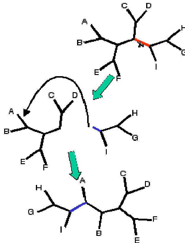
Figure 14 – SPR (Subtree Pruning and Regrafting)
