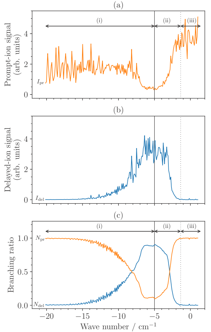
FIG. 2. Prompt (a) and delayed (b) \text{Mg}^+ ion signal obtained for a dc field of -49 mV/cm when scanning the second laser in the vicinity of the \text{Mg}^+(3s^2S_{1/2}) ionization threshold. The regions labeled (i)–(iii) and separated by vertical lines are the regions where the dominant mechanisms for the production of prompt ions are (i) the autoionization of the 3p_{3/2}nl core-excited Rydberg states, (ii) the PFI of 3s_{1/2}nl Rydberg states, and (iii) direct ionization into the 3s^2S_{1/2} ionization continuum (see text and details). (c) Branching ratios for the production of the prompt ( N_{\text{pr}} ) and delayed ( N_{\text{del}} ) ions. The wave-number scale is given relative to the field-free ionization threshold.
