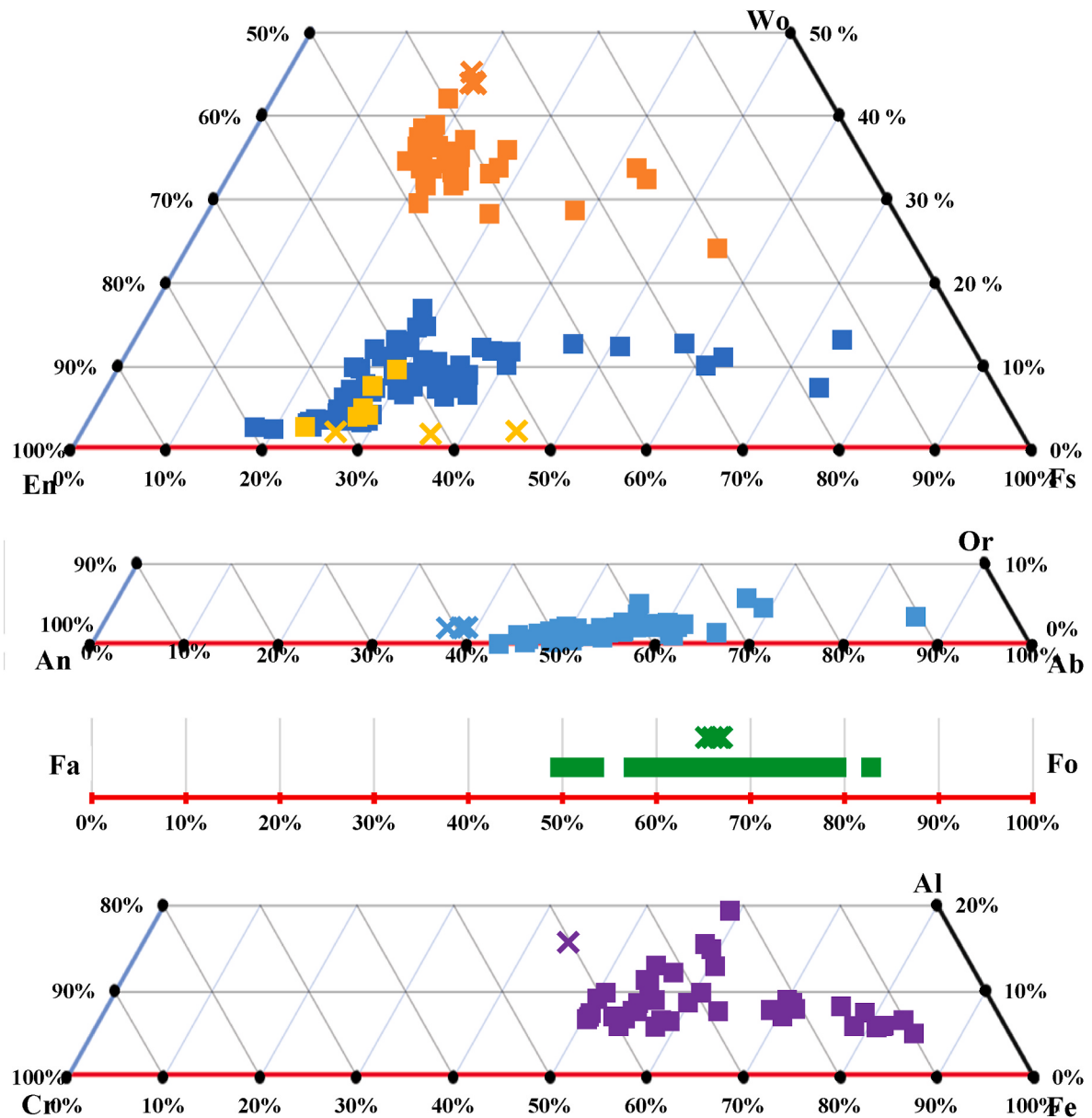
Fig. 1. Endmember comparison between our pure mineral phases (crosses) and considered shergottites (squares) for (top to bottom) high-Ca cpx (orange), low-Ca cpx (dark blue), opx (yellow), plagioclase (light blue), olivine (green), and chromite (purple). Data gathered from The Martian Meteorite Compendium and references within (Balta et al., 2015; Steele and Smith, 1982; Papike et al., 2009; Treiman, 1994; Gleason et al., 1997; Harvey et al., 1993; Hsu et al., 2004; Lin et al., 2005; Jiang and Hsu, 2012; Usui et al., 2010; Basu Sarbadhikari et al., 2009; Stöfler et al., 1986).
