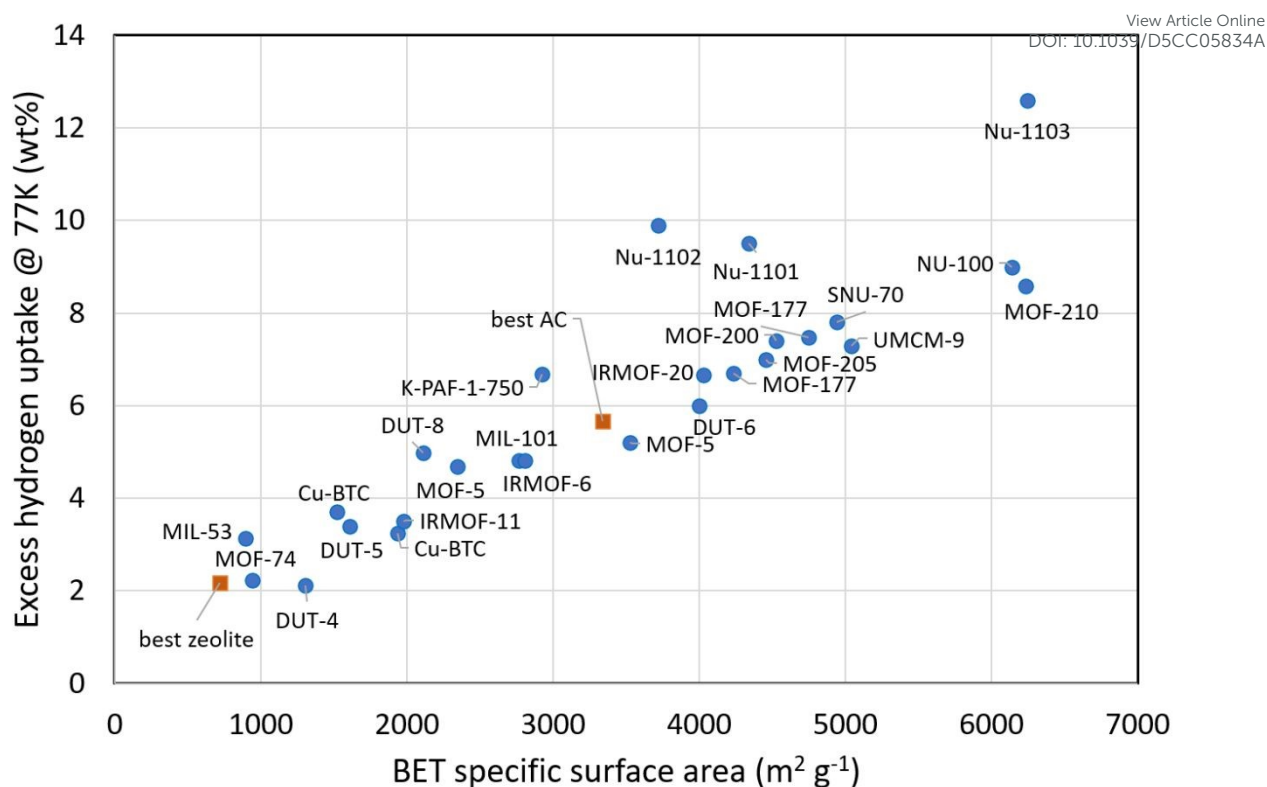
Figure 2. Excess gravimetric hydrogen uptake for various MOFs at 20 bar or above and 77 K (data shown as circles). For comparison the data for the best zeolite and activated carbon (AC) is also included (data shown as squares). The slope is approximately 1 wt% per 500 m 2 /g, showing Chahine's Rule. Adapted from Broom et al. 20 with permission from Springer, Applied Physics A | Volume 122 | Jan 2016 | 151, copyright 2026 under the terms of the Creative Commons Attribution 4.0 International License ( http://creativecommons.org/licenses/by/4.0 ), with additional data from Li et al. 34 and Ahmed et al. 35
