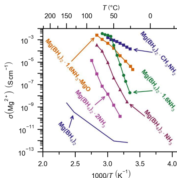
Figure 4 Magnesium ionic conductivity as a function of temperature for derivatives of magnesium tetrahydridoborate. Raw data presented in Figure 4 is published in reference 17, 145 and 148.
