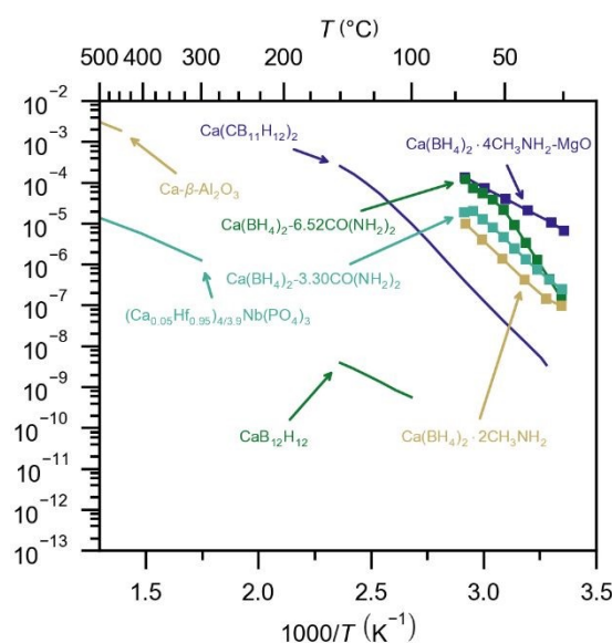
Figure 5. Calcium ionic conductivity as a function of temperature for derivatives of calcium tetrahydridoborate compared to that of known oxide, phosphate and hydrido- closo -(carba)borate based electrolytes. Raw data presented in Figure 5 is published in reference 155-157.
