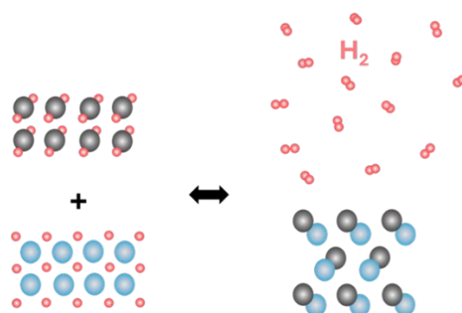
Figure 3 Illustration of reactive hydride composites (RHC). Initially the hydrides release hydrogen and then react and form a new compound. This new compound may facilitate hydrogen uptake as compared to the individual hydrides.
