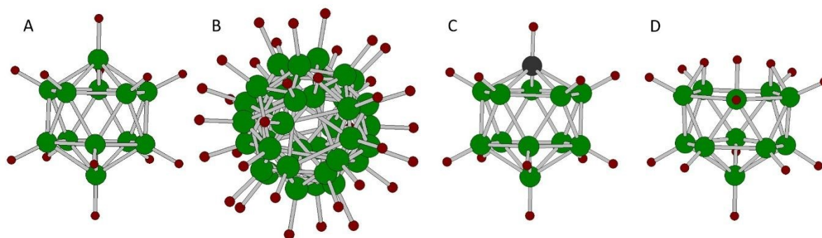
Figure 6. Structure of selected hydridoborate anions. A) Dodecahydrido- closo -dodecaborate( 2- ) anion, \text{B}_{12}\text{H}_{12}^{2-} in an ordered structure. B) Dodecahydrido- closo -dodecaborate( 2- ) anion, \text{B}_{12}\text{H}_{12}^{2-} in a disordered structure where the anion is statistically or dynamically distributed over two crystallographic positions. C) Dodecahydrido- closo -monocarbododecaborate( 1- ), \text{CB}_{11}\text{H}_{12}^- . D) Tetradecahydrido- nido -undecaborate( 1- ), \text{B}_{11}\text{H}_{14}^- .
