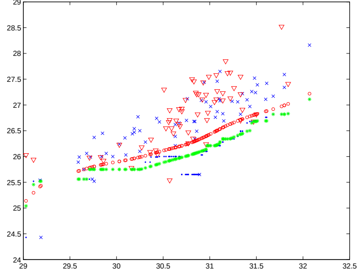
Figure 4: Estimated conditional first quartile for the quasars data. The estimators \tilde{m}^T(x) , \hat{m}_{alt}^T(x) and \hat{m}^T(x) are indicated by \cdot , \circ and * respectively. Uncensored data points are represented by \times , and (left) censored observations by \nabla .
