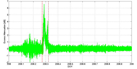
Fig. 10. Excess attenuation at Ka band at UTM, Malaysia
