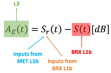
Fig. 2. Excess Attenuation Algorithm
