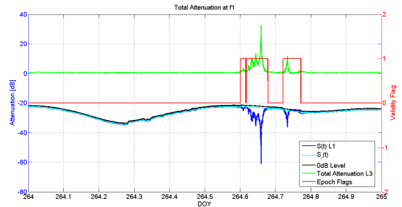
Fig. 6. Example of processed data in Graz, Austria
