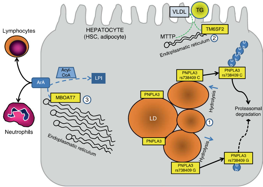
Fig. 2 Putative functions of proteins encoded by PNPLA3 , TM6SF2 , and MBOAT7 . All proteins encoded by the three genes are enzymes related to lipid/fatty acid turnover are expressed in the liver tissue. The functional link to hepatocarcinogenesis is as yet unknown. PNPLA3 [1] is an enzyme with both triacylglycerol lipase and acylglycerol O-acyltransferase activities and plays an important role in the balance of energy usage/storage in adipocytes, hepatocytes, and likely, hepatic stellate-cells [9, 34]. Expression of PNPLA3 protein and mRNA increases the following food intake. The polymorphic variant ( PNPLA3 rs738409 G) is a loss-of-function mutation, in which structural alteration of the substrate-binding groove leads to lower substrate accessibility, and thus less triglyceride hydrolysis [35]. Also, the mutant variant rs738409 G, which locates on lipid droplets, evades proteasomal degradation by disrupting ubiquitylation [36]. Consequently, the mutant PNPLA3 variant accumulates resulting in impaired triglyceride mobilization [36]. TM6SF2 [2] is only incompletely characterized functionally, but appears to modulate hepatic lipoprotein export and lipidation of very low-density lipoproteins (VLDL). A functional link between TM6SF2 and the microsomal triglyceride transfer protein (MTTP) jointly regulates the assembly and secretion of VLDL and triglycerides (TG) from liver cells into the bloodstream. The polymorphic variant of the TM6SF2 gene (rs58542926 T) encodes a loss-of-function TM6SF2 protein, which impairs VLDL export and, thus, increases intracellular lipids, but decreases the circulating serum VLDL, LDL, and triglyceride levels. These opposing functional differences result in distinct risk effects on steatosis and liver fibrosis (increased with variant rs58542926 T) [31] and on cardiovascular risk (increased with wild type rs58542926 C) [32]. MBOAT7 [3] is a lysophosphatidylcholine acyltransferase, and as such is involved in membrane phospholipid remodeling. It catalyzes the transfer of acyl-CoA to lysophosphatidylcholine (LPI) with a strong propensity for arachidonoyl-CoA as the acyl donor [37]. Consequently, it may regulate the mechanisms by which pro-inflammatory free arachidonic acid (ArA) and eicosanoid levels are regulated. Increased availability of ArA leads to inflammatory signaling by prostaglandins and leukotrienes, which are potent chemoattractants of inflammatory cells. The MBOAT7 rs641738 T allele leads to lower hepatic MBOAT7 protein expression and changes in plasma phosphatidylcholine profiles consistent with a loss of function variation [38]
