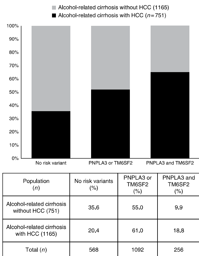
Fig. 1 Proportion of cases with alcohol-related cirrhosis and HCC by carriage of the risk variants in PNPLA3 and TM6SF2
