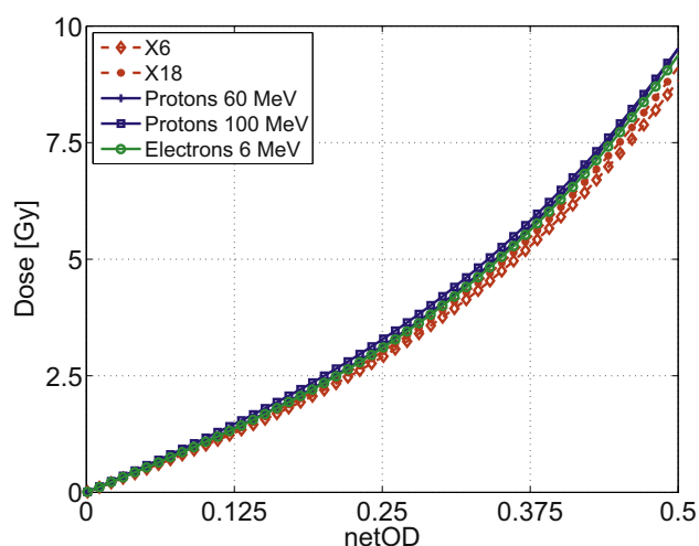
Figure 5 Superposition of red channel calibration curves for each modalities: 6 MV (diamonds, dotted line), 18 MV (stars, dotted line), 60 MeV protons (plus signs, solid line), 100 MeV protons (squares, solid line) and 6 MeV electrons (circles, solid line). (For interpretation of the references to color in this figure legend, the reader is referred to the web version of this article.)
